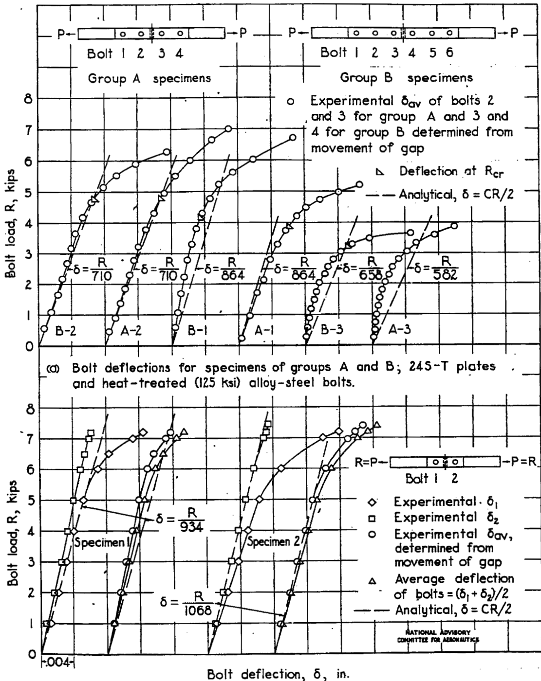
Figure 16.- Comparison of experimental and analytical bolt deflections.
