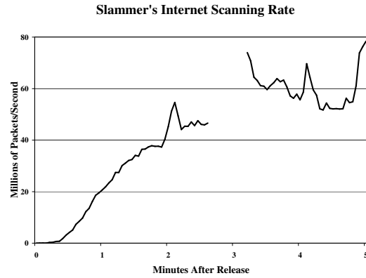
Figure 1: Slammer’s Internet scanning rate, as measured at the University of Wisconsin Tarpit Network
