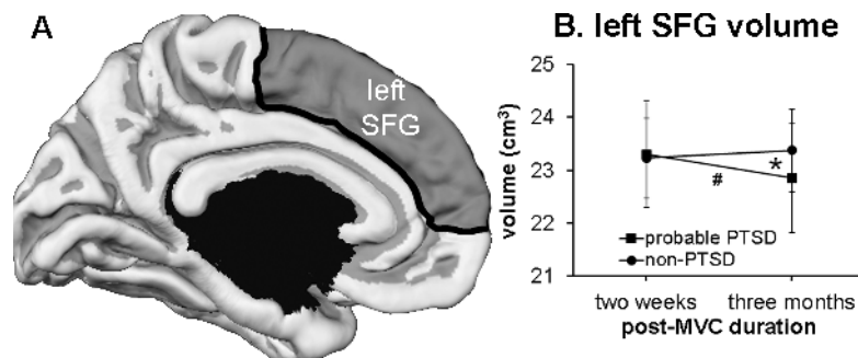
Fig 3. Volume of left SFG. (A) parcellation of left SFG (shaded in gray) in FreeSurfer partially overlaps with location of the dmPFC activation cluster. (B) Volume of left SFG at two weeks and three months after MVC. *: indicates significant effect of time by group interaction. #: indicates significant decrease in left SFG volume in probable PTSD group over time. The error bars indicate the standard error of the mean.
