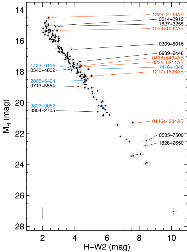
Figure 8. Trends of absolute H -band magnitude with H-W2 color for all objects from Table 7 that fall within 20 pc of the Sun ( \pi_{\text{abs}} \geq 50 mas). Known binary systems are circled and labeled in red, and known subdwarfs are circled and labeled in blue. Other objects falling significantly above or below the mean trend are labeled in black. The light gray bar at the lower left shows the size of the 0.75 mag offset expected for an equal-magnitude binary.
