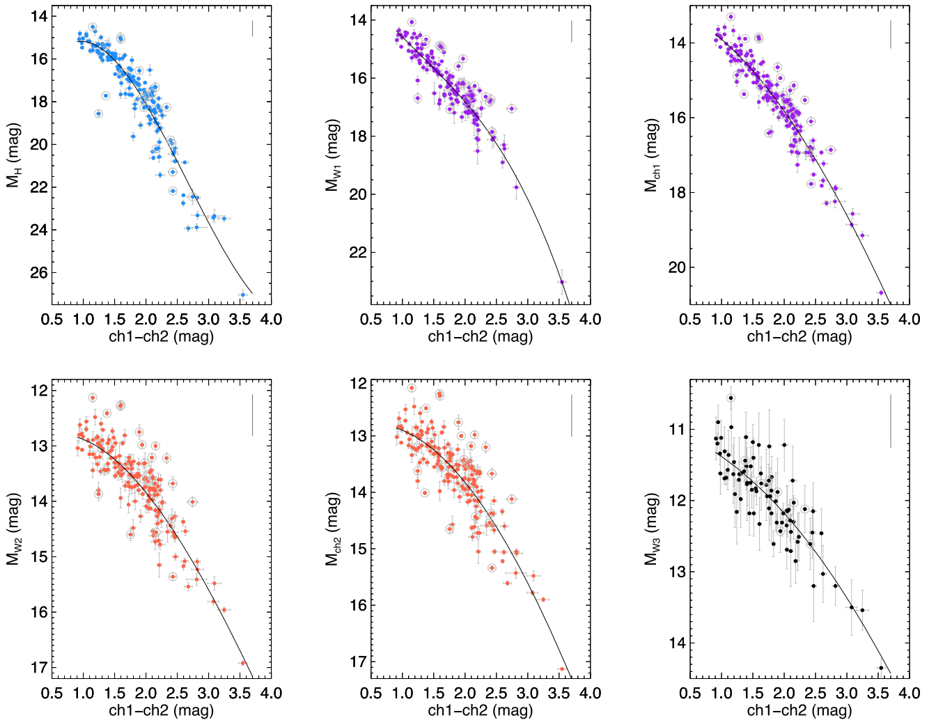
Figure 6. Trends of absolute magnitude with \text{ch1}-\text{ch2} color for all objects from Table 7 that fall within 20 pc of the Sun ( \tau_{\text{abs}} \geq 50 mas). The top row shows trends with absolute H -band magnitude (light blue) and the similar absolute W1 and ch1 magnitudes (purple). The bottom row shows trends with the similar absolute W2 and ch2 magnitudes (orange red) and the absolute W3 magnitude (black). Polynomial fits to the relations are shown by the black curves, and the functional forms are presented in Table 8. Points ignored by the fitting (see Section 8.3) are circled in gray. The light gray bar at the upper right of each panel shows the size of the 0.75 mag offset expected for an equal-magnitude binary.
