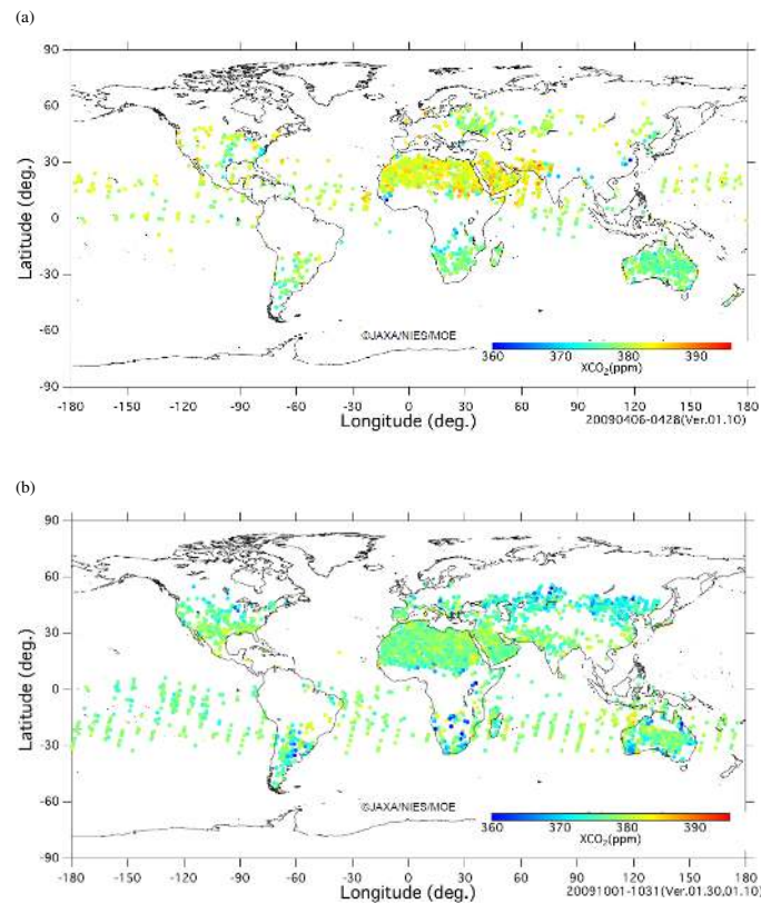
Fig. 2. Global distribution of GOSAT SWIR X_{CO_2} for (a) April and (b) October in 2009.
