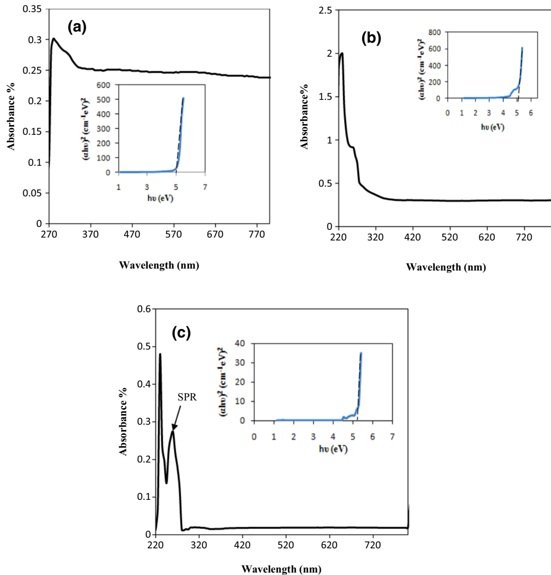
Fig. 3 Optical absorbance of fresh colloidal Al 2 O 3 NPs prepared at different laser fluences: a 3.5 J/cm 2 , b 5.2 J/cm 2 , c 7.3 J/cm 2 . Inset shows the (\alpha h\nu)^2 versus photon energy plot
