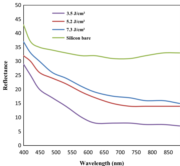
Fig. 10 Effect of laser fluence on the optical reflectance of nanostructured alumina films deposited on silicon photodiode
