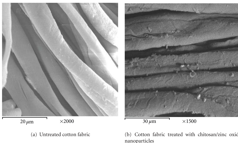
FIGURE 6: SEM of cotton fabric treated with chitosan/ZnO nanoparticles.
