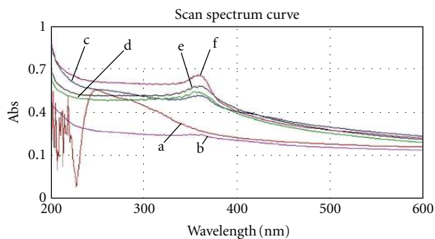
FIGURE 1: UV-vis absorbance spectra of chitosan and chitosan/ZnO nanoparticles at different concentrations. (a) chitosan, (b) chitosan/ZnO (0.1%), (c) chitosan/ZnO (0.25%), (d) chitosan/ZnO (0.5%), (e) chitosan/ZnO (0.75%) and (f) chitosan/ZnO (1%).
