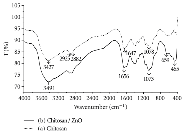
FIGURE 3: FTIR of chitosan (a) and chitosan/ZnO nanoparticles (b).
