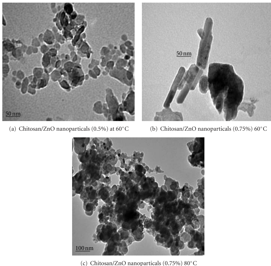
FIGURE 4: TEM photographs of chitosan/ZnO nanoparticles.
