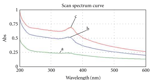
FIGURE 2: UV-vis absorbance spectra of chitosan and chitosan/ZnO (0.75%) nanoparticles at different temperatures (a) at 40°C, (b) at 60°C, and (c) at 80°C.
