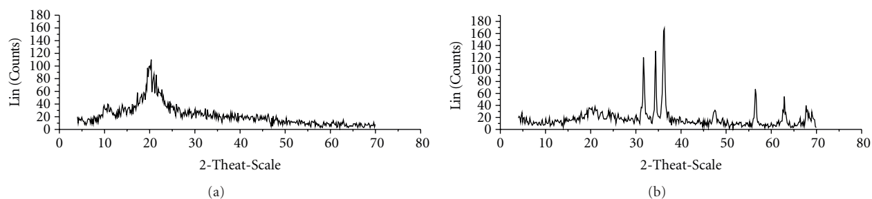
FIGURE 5: X-ray diffraction patterns of chitosan (a) and chitosan/ZnO nanoparticles (b).
