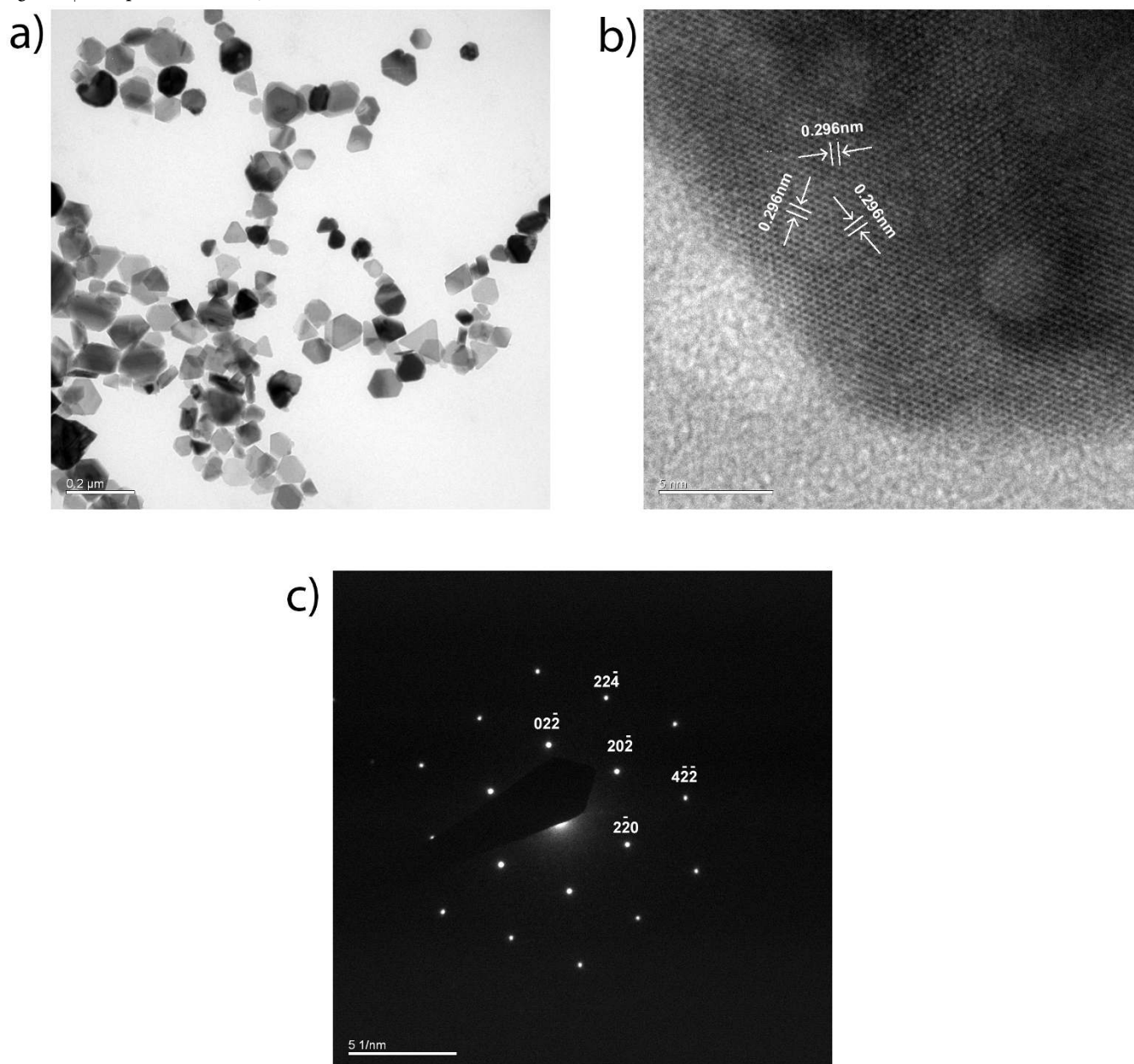
Figure 2 | (a) Low magnification TEM image of \text{Fe}_3\text{O}_4 nanosheets; (b) HRTEM of \text{Fe}_3\text{O}_4 nanosheets; (c) SAED pattern of \text{Fe}_3\text{O}_4 nanosheets. The scale bars are 0.2 \mu\text{m} , 5 nm, and 5 1/nm respectively.
