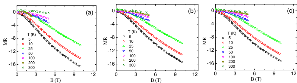
Figure S5. The magnetoresistance as a function of B at different temperatures for (a) CNT yarn, (b) Electrochemically prepared CNT-PPy yarn, and (c) Chemically prepared CNT-PPy yarn.
