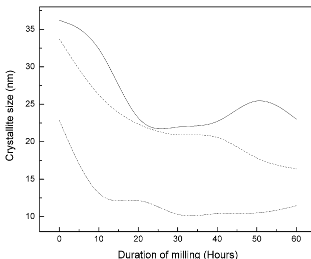
Fig. 5 Variation in crystallite size with milling time. (—) indicates quartz peak at 2\theta = 20.86^\circ , (- - -) indicates mullite peak at 2\theta = 40.858 and (----) indicates iron oxide peak at 35.29^\circ .
