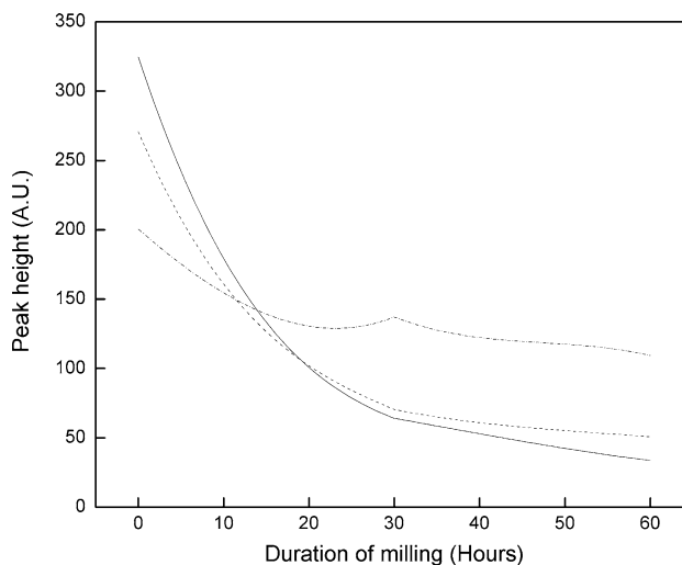
Fig. 6 Variation in peak height with milling time. (—) indicates quartz peak at 2\theta = 20.86^\circ , (- - -) indicates mullite peak at 2\theta = 40.858 and (----) indicates iron oxide peak at 35.29^\circ
