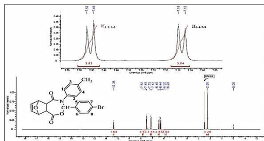
Figure 4: 1 H-NMR spectrum for Compound [E 3 ].
