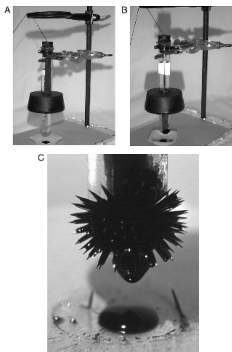
Figure 11. The leaping ferrofluid demonstration. (A) The magnets are in the raised position. (B) The magnets are in the lowered position. (C) Ferrofluid spiking at the end of the test tube, which occurs when the magnets are in the lowered position.
