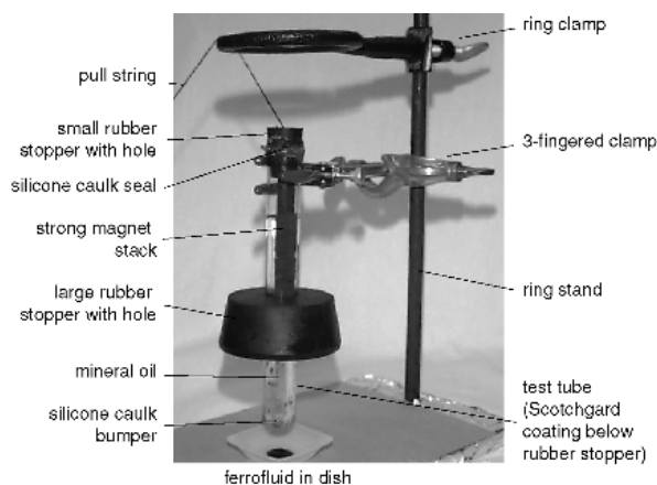
Figure 9. Construction of the "leaping ferrofluid" demonstration.
