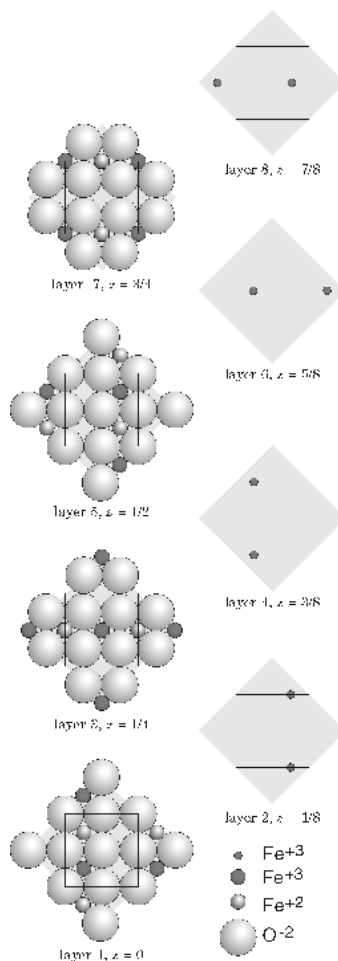
Figure 3. The layer sequence of magnetite (see ref 4b, Chapter 3, for a discussion of layer sequences). The larger gray square represents the cross-section of the conventional cubic unit cell; the smaller, black-outlined square represents the cross-section of an alternate, smaller tetragonal unit cell. The arrangement of the atoms is the same in both. \text{Fe}^{3+} is represented by circles of different sizes: large circles represent iron in octahedral coordination, small circles represent iron in tetrahedral coordination.
