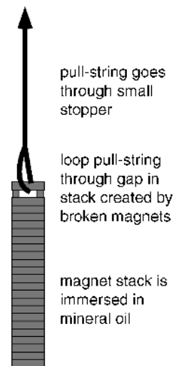
Figure 10. Construction of the magnet stack used in the "leaping ferrofluid" demonstration.
