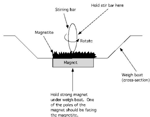
Figure 5. The final ferrofluid preparation step. Remove the magnetite from both ends of the stirring bar by grasping the bar in the center, touching each end in turn to the weighing boat above the strong magnet, and rotating the stirring bar until all of the magnetite adheres to the weighing boat through attraction to the strong magnet beneath the boat.
