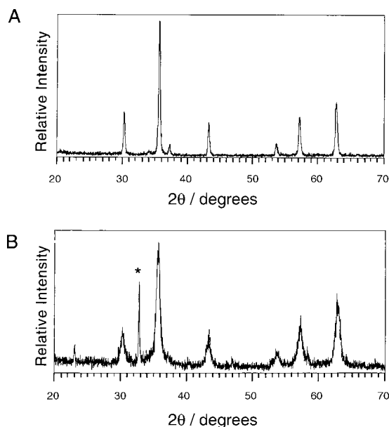
Figure 8. (A) X-ray powder diffraction pattern of commercially available magnetite. (B) X-ray powder diffraction pattern of the magnetite synthesized by the technique outlined in this paper: Using eqs 2 and 3, the average particle size is about 14 nm. The peak used in the calculations was at 2\theta = 35.6^\circ (Miller indices, (311)). The asterisk indicates an impurity peak.
