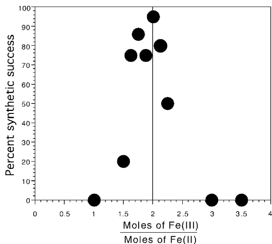
Figure 7. Percent success of the ferrofluid synthesis as a function of iron chloride solution mole ratios for a group of \sim 250 pairs of undergraduates performing the experiment during the third week of class. Most of the trials were conducted with the 2:1 \text{Fe}^{3+}/\text{Fe}^{2+} ratio.
