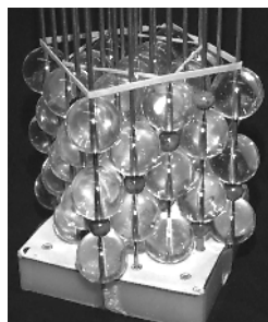
Figure 4. Model of the cubic unit cell of \text{Fe}_3\text{O}_4 , built with the ICE Solid State Model Kit (11).
