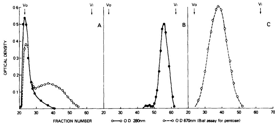
Fig 1 Gel filtration through CL-4B Sepharose of. (A) HIB Ps-Johnson-BSA-33 conjugate, (B) AH-BSA-33, and (C) Johnson HIB Ps. The protein content of the fractions was measured by recording the absorbance at 280 nm and the polysaccharide was measured by the Bial reaction (absorbance at 670 nm) (44). The fractions 22-28, containing both protein and polysaccharide components, were pooled, dialyzed against saline, and sterile-filtered for further studies and have been designated as Johnson-BSA-33 Vi, total volume of column, Vo, void volume
