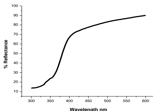
Fig. 3. UV-Vis.DRS of T
