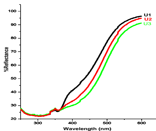
Fig.4 UV-Vis.DRS of N doped titania catalysts
