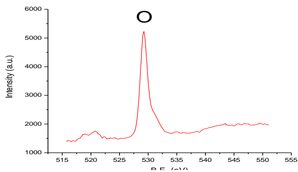
Fig.11 O 1s spectrum of sample U2
