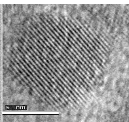
Fig.8 HRTEM image of U2
