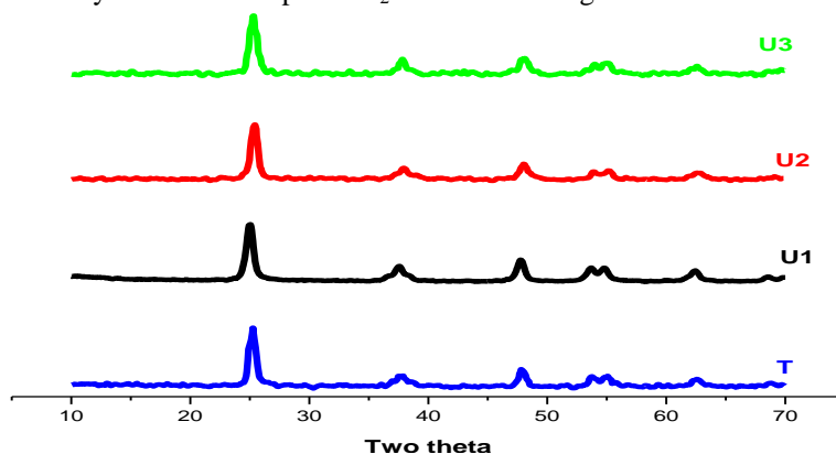
Fig.2 XRD pattern of N doped titania
