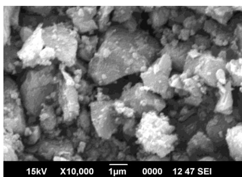
Fig.5 SEM image of undoped titania(T)
