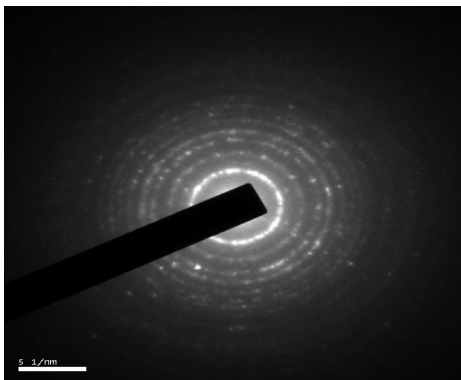
Fig.9 SAED image of U2
