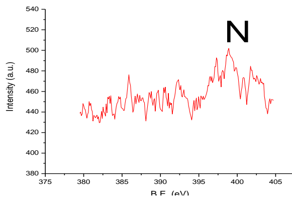
Fig. 12 N 1s spectrum of sample U2
