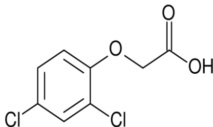
Fig. 1 Structure of 2,4-D
