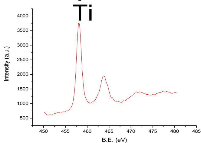
Fig.10 Ti 2p spectrum of sample U2
