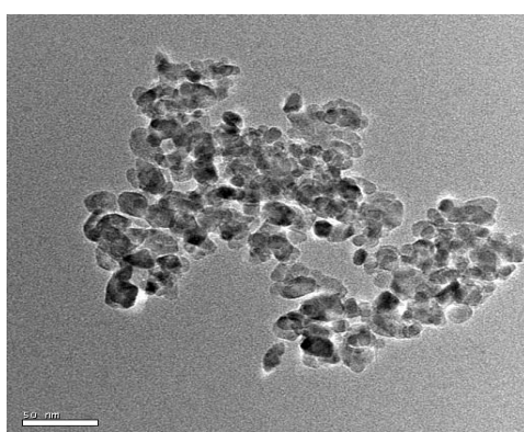
Fig.7 TEM image of U2
