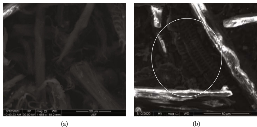
FIGURE 2: SEM images of sisal fibers: (a) untreated (USF) and (b) treated (TSF).
