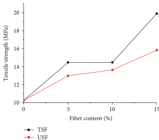
FIGURE 7: Tensile strength of composites from treated and untreated sisal fiber.
