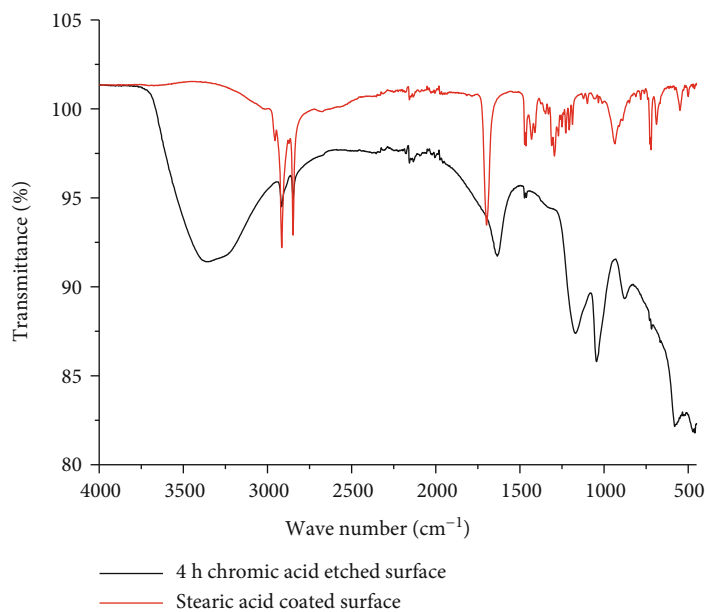
FIGURE 12: FTIR spectrum of composite material before and after surface modification.
