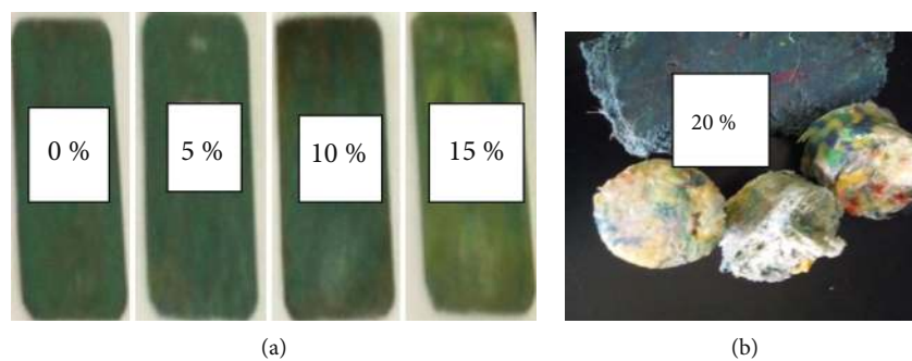
FIGURE 4: Sisal fiber-reinforced polypropylene composite: (a) 0-15% fiber content and (b) 20% fiber content.
