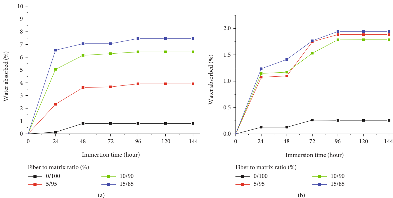
FIGURE 15: Water absorption percentage (%) of (a) unmodified composites and (b) modified composite at different time intervals.
