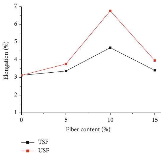
FIGURE 8: Elongation of composites from treated and untreated sisal fiber.
