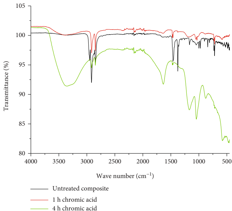
FIGURE 10: FTIR spectra of untreated and chromic acid etched composite for 1 and 4 h.
