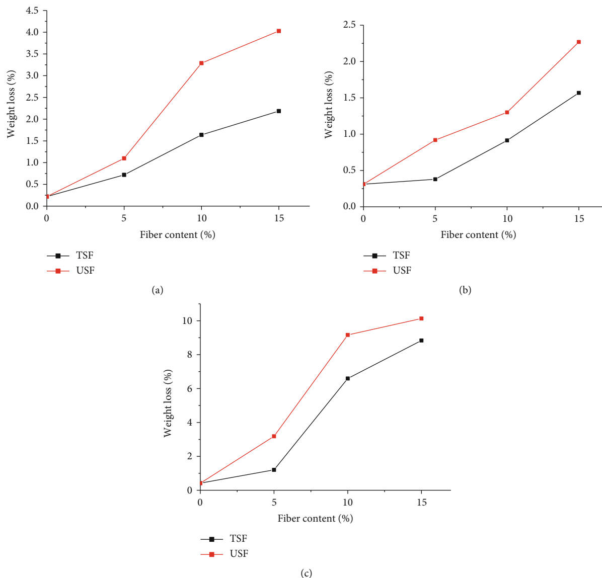
FIGURE 9: Percentage weight loss of composites in (a) 30% NaOH, (b) 30% HCl, and (c) 30% H 2 SO 4 .
