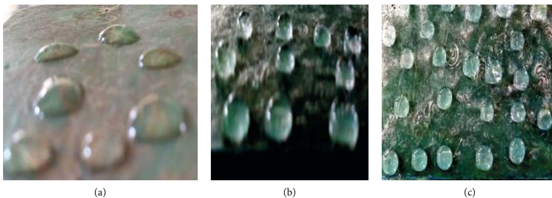
FIGURE 13: Water droplets on composite material (a) before surface modification, (b) chromic acid etched, and (c) stearic acid-modified surface.
