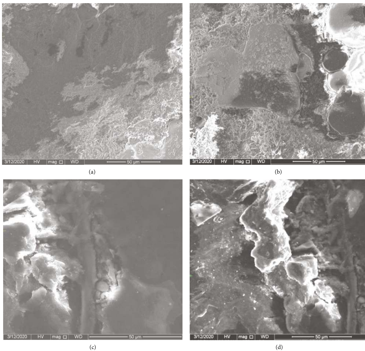
FIGURE 5: SEM images of composite (a) 0%, (b) 5%, (c) 10%, and (d) 15% fiber loading.
