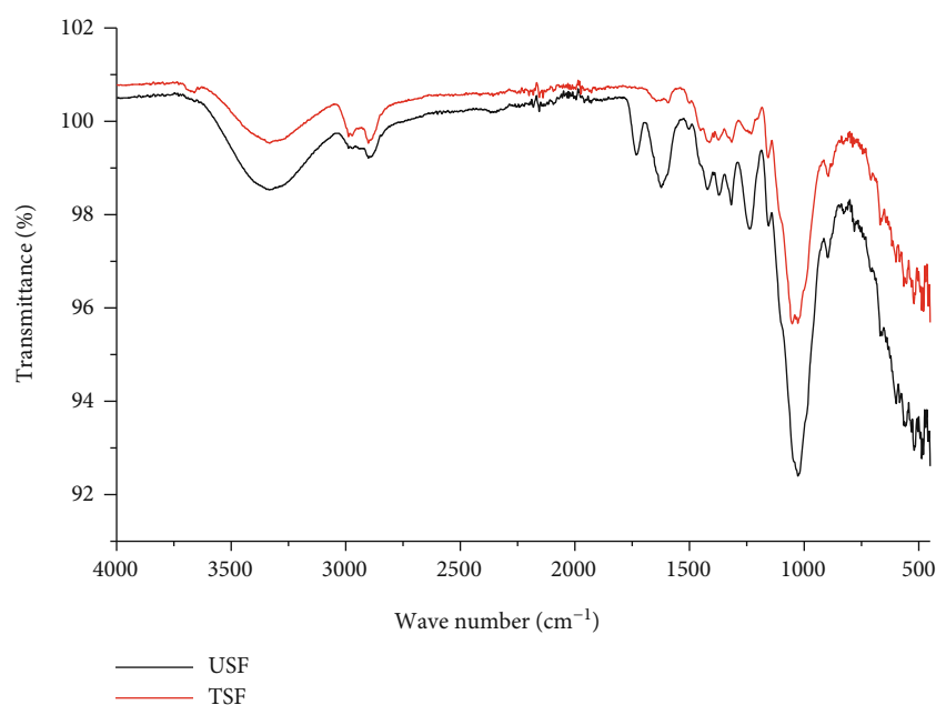
FIGURE 3: FTIR spectra of untreated and treated sisal fibers.
