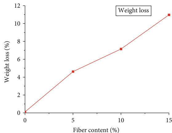
FIGURE 6: Percentage weight loss of the composites with different fiber loading.
