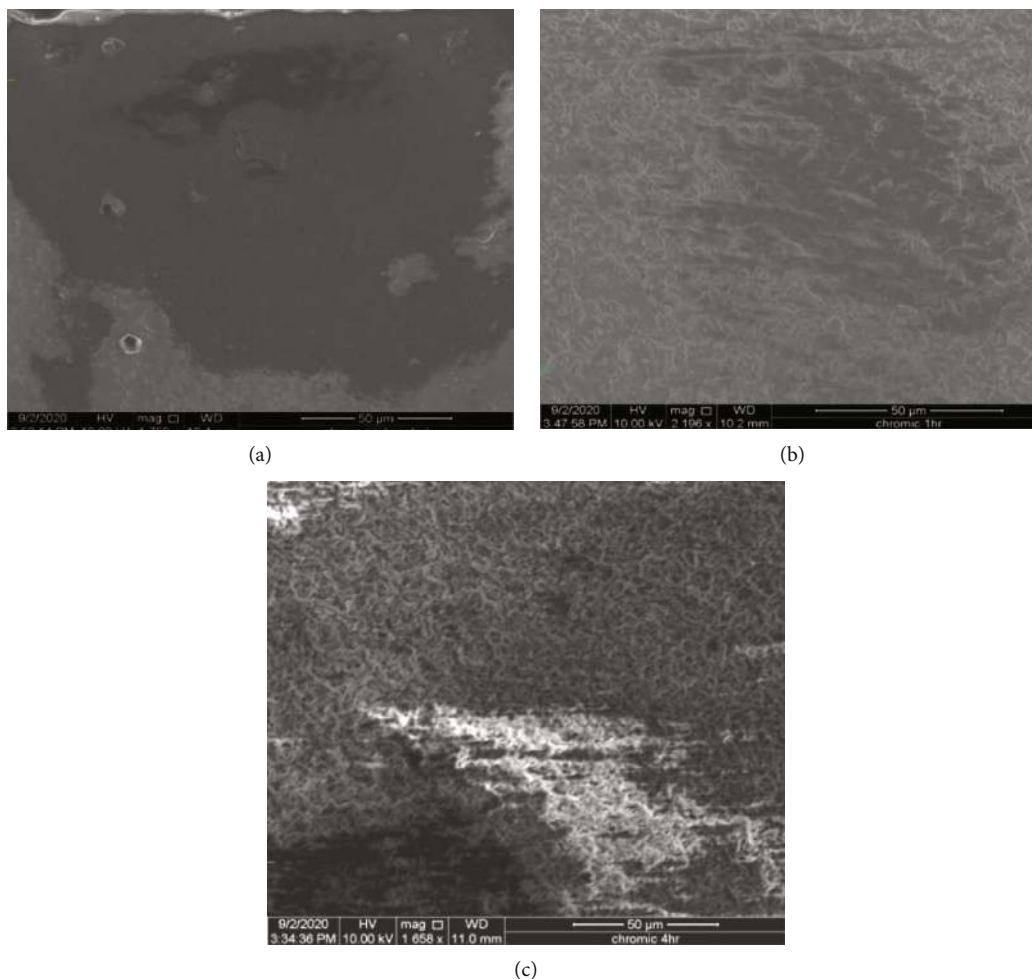
FIGURE 11: SEM images of a composite (a) before chromic acid etching and (b) after etching for 1 h and (c) for 4 h.
