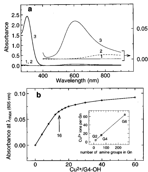
Figure 1. (a) Absorption spectra of 0.6 mM \text{CuSO}_4 in the presence (solid line, curve 3) and in the absence (dashed line, curve 2) of 0.05 mM G4-OH. Curve 1 is the absorption spectrum of 0.05 mM G4-OH vs water. (b) Spectrophotometric titration plot: absorbance at the peak maximum of 605 nm as a function of the number of \text{Cu}^{2+} ions per G4-OH. The initial concentration of G4-OH was 0.05 mM. The inset shows the relationship between the number of \text{Cu}^{2+} ions complexed within \text{G}_n\text{-OH} and the number of 3^\circ amine groups within \text{G}_n\text{-OH} . The titration end point is estimated as the extrapolated intersection of the two linear regions of the curve before and after the equivalence point. The optical path length was 1 cm, the temperature was 20 \pm 2^\circ\text{C} , and unbuffered aqueous \text{CuSO}_4 (pH \sim 5.1 ) was used to titrate the unbuffered aqueous dendrimer solution (pH \sim 8.1 for \text{G}_n\text{-OH} and pH \sim 9.0 for \text{G}_4\text{-NH}_2 ).
