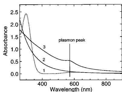
Figure 2. Absorption spectra of a solution containing 0.6 mM \text{CuSO}_4 and 0.05 mM G4-OH before (dashed line, curve 1) and after (solid line, curve 2) reduction with a 5-fold molar excess of \text{NaBH}_4 . Curve 3 was obtained under the same conditions as those for curve 2 except 0.05 mM G4- \text{NH}_2 was used in place of G4-OH.
