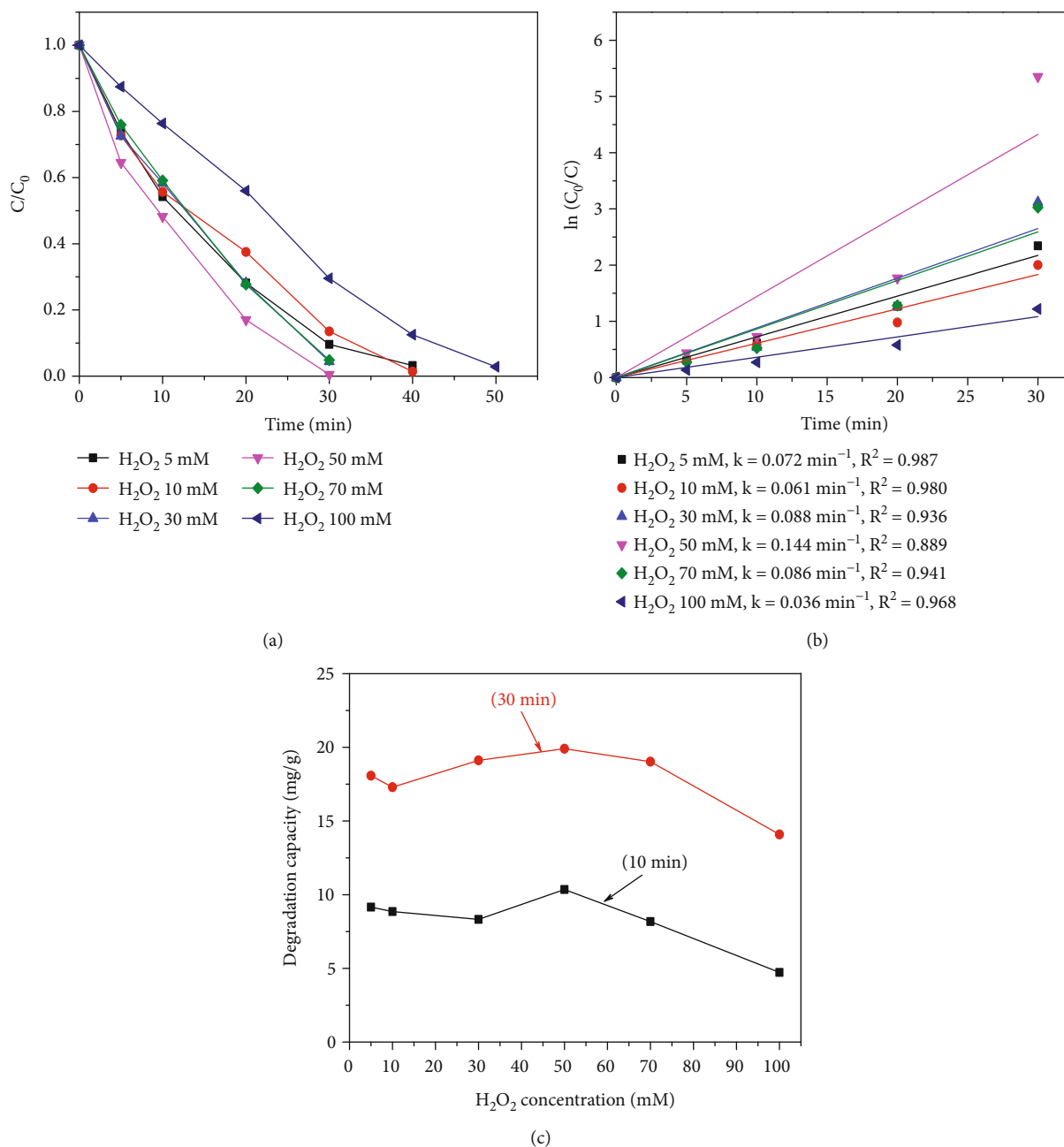
FIGURE 13: (a) Effect of initial \text{H}_2\text{O}_2 concentration on degradation of tartrazine, (b) the kinetic curves, and (c) the DC with different \text{H}_2\text{O}_2 concentrations. The reaction conditions: catalyst dosage of 0.5 g/L, TA concentration of 10 mg/L, pH solution of 6.0, and Hg lamp 250 W.
