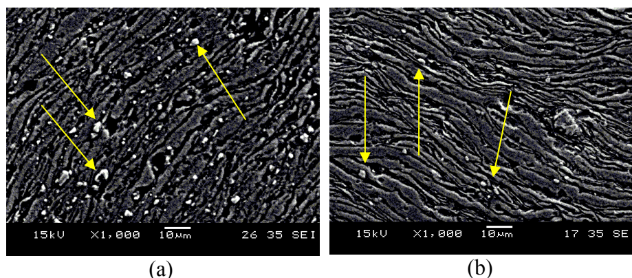
Figure 3.3 - Distribution of the strengthening phase in the composite reinforced with 10% (a) of aluminum nitride (AlN) subjected to high energy ball milling for 60 minutes (a) after compaction and sintering. (b) 10% bulk silicon nitride ( \text{Si}_3\text{N}_4 ) subjected to high energy ball milling for 60 minutes (a, b) after compaction and sintering.
