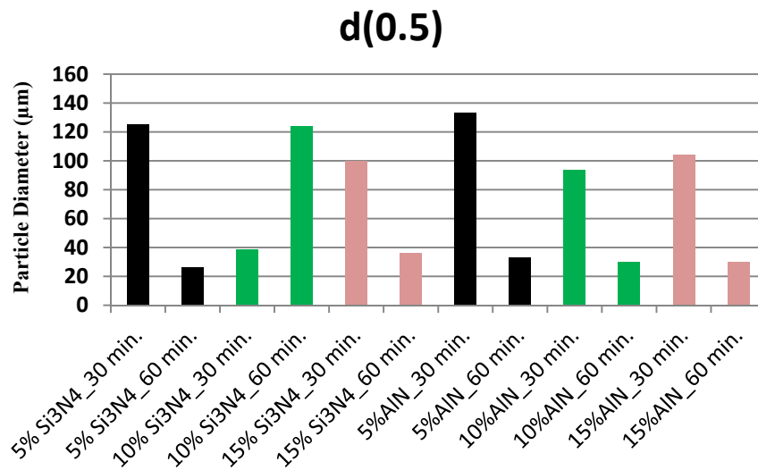
Figure 3.1 - The particle diameter of the composite reinforcement with 5, 10 and 15% bulk silicon nitride and aluminium nitride subjected to 30 and 60 minutes of grinding, respectively.
