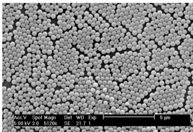
FIG. 6. SEM picture of the system PMMA-NBD8.
