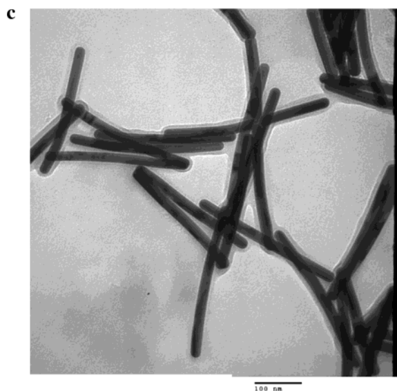
Figure 2. TEM images of (a) Au nanorods, (b) polystyrene-coated Au nanorods, and (c) silica-coated Au nanorods. Scale bars = 100 nm.
