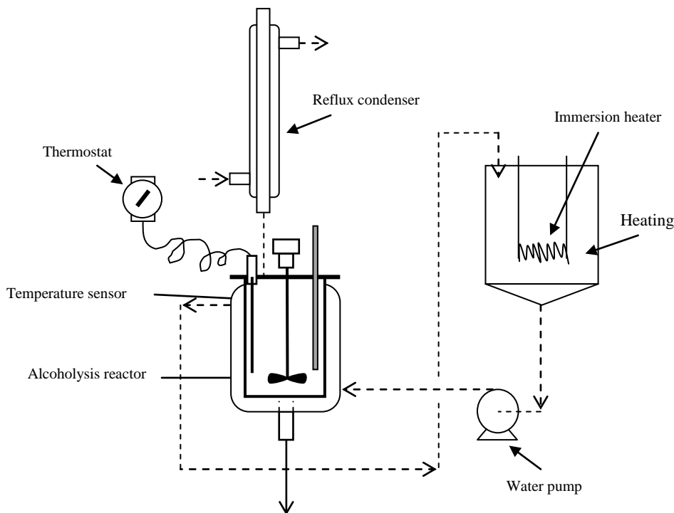
Fig. 2 Alcoholysis process unit
