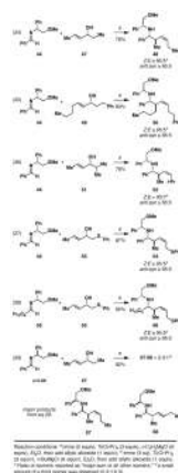
Figure 14. Double asymmetric reductive cross-coupling.
