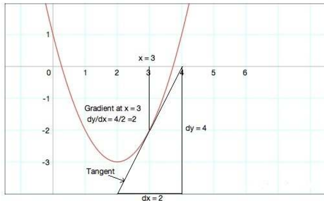
Figure 8: A representation of y = x^2 - 4x + 1 , with a tangent drawn at x = 3 .
