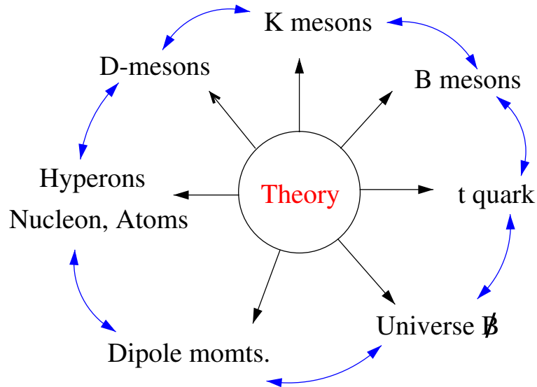
Figure 16. CP-Violation
