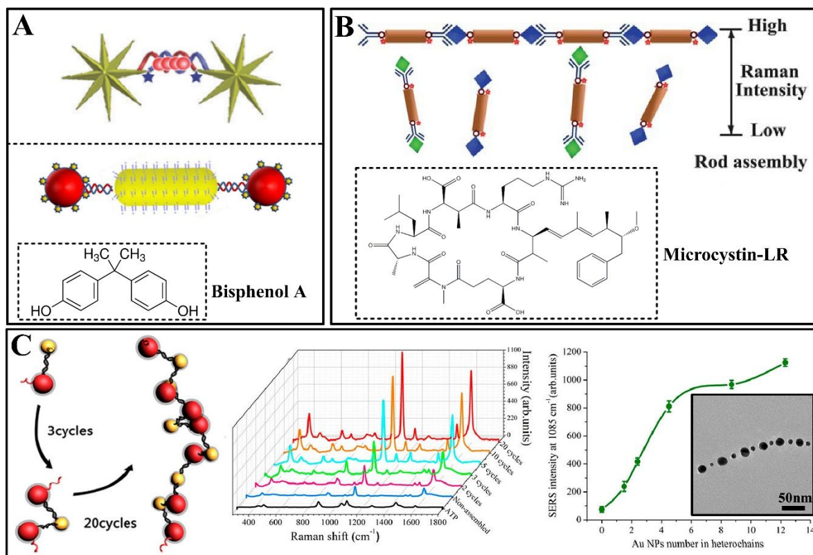
Figure 37. (A) Surface-enhanced Raman scattering (SERS) active gold nanostar dimer for mercury ion detection (top) and gold nanoparticle–nanorod heteroassemblies for bisphenol A detection (bottom). Adapted with permission from refs 709 and 704. Copyrights 2013 Royal Society of Chemistry and 2016, Elsevier B. V., respectively. (B) SERS active gold nanorod assembly for toxin detection. Adapted with permission from ref 559. Copyright 2012 Royal Society of Chemistry. (C) Plasmonic nanoparticle heterochains and SERS enhancement properties. Adapted from ref 710. Copyright 2013 American Chemical Society.
