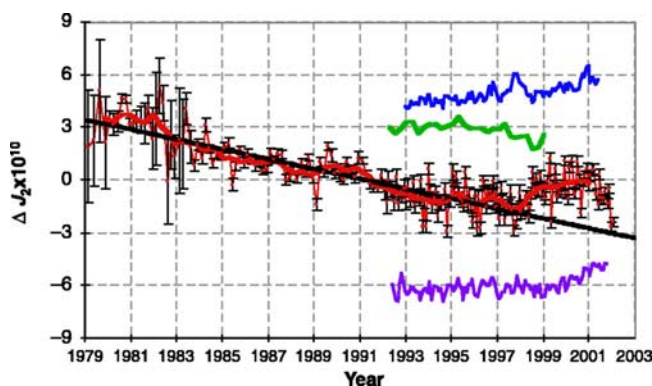
Figure 15. Monthly variations of the Earth's gravitational oblateness ( J_2 ) based on satellite laser ranging data to numerous geodetic satellites from 1979 to 2001. Reprinted with permission from Cox and Chao [2002]. Copyright 2002 American Association for the Advancement of Science.
