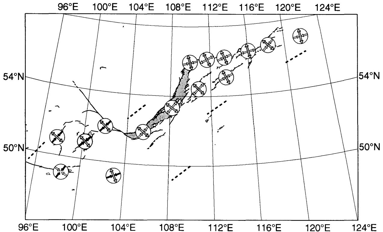
Figure 4. Map view of main horizontal stress directions in the Baikal rift (see Table 2). Grey arrows are \sigma_3 ; open divergent arrows are \sigma_2 when R > 0.5 ; open convergent arrows are \sigma_2 when R < 0.5 ; solid arrows are \sigma_1 . Thick dashed line is regional S_{Hmax} direction after Tapponnier and Molnar [1979] and Zoback [1992].
