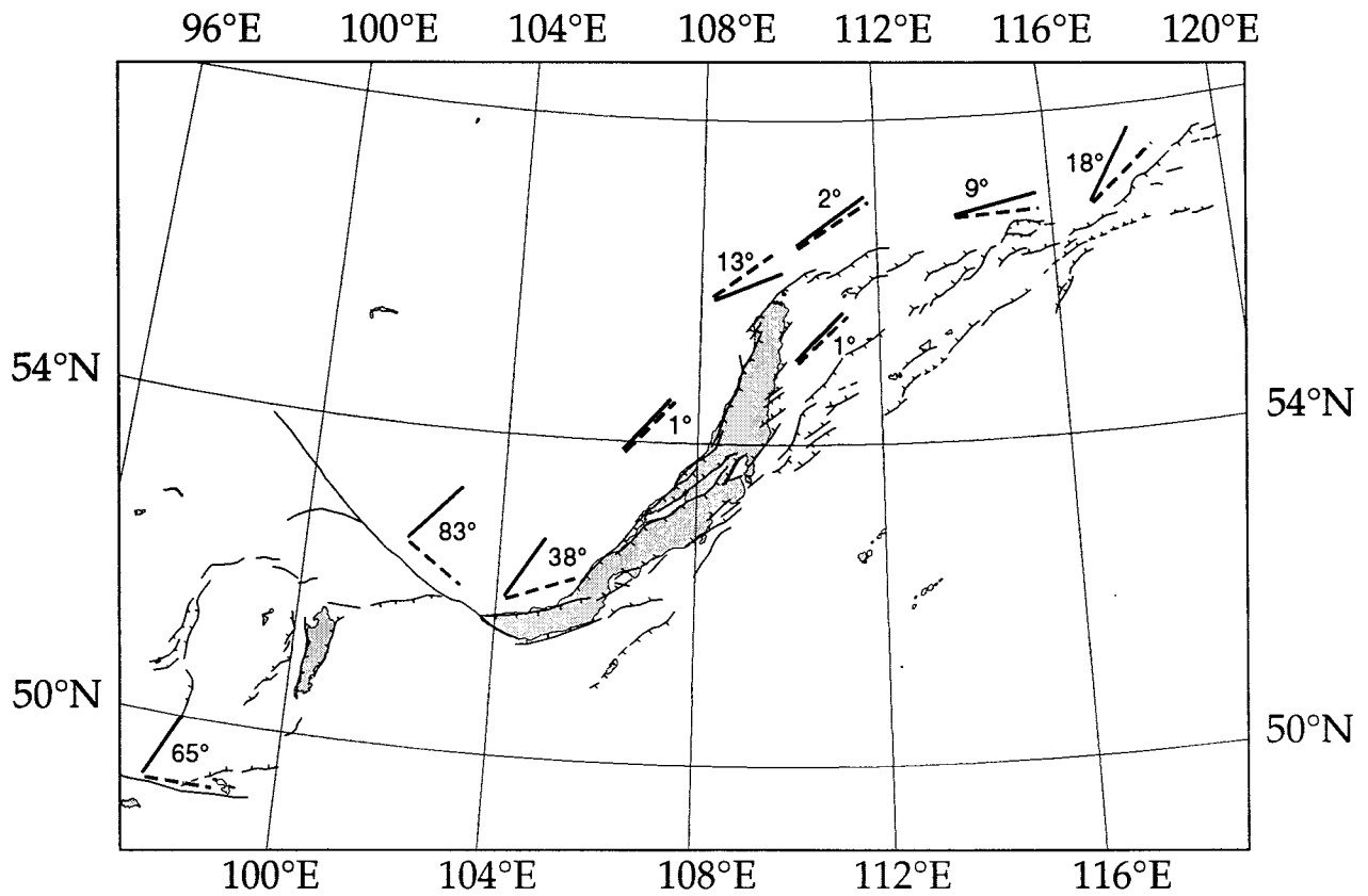
Figure 8. Map of angular differences between S_{Hmax} directions (thick lines) and active fault strikes (dashed lines), referred to the active fault pattern of the rift area (thin lines).
