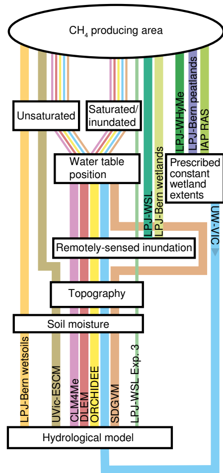
Fig. 6. Conceptual overview of how the participating models derive their “CH 4 producing area” (MPA). Each model (and in some cases, version) is represented by a different colour. The flow of a particular model starts with the model’s name and ends at the “CH 4 producing area”. The simplest models rely on “Prescribed constant wetland extents” to define their MPAs (LPJ-WhyMe, LPJ-Bern peatlands, IAP-RAS), whereas UW-VIC uses “Prescribed constant wetland extents” only as maximal boundaries. LPJ-WSL and LPJ-Bern wetlands use remotely sensed inundation directly. “Soil moisture” is exclusively simulated by a “Hydrological model” and is used to either derive “Unsaturated” MPAs directly (LPJ-Bern wetsoils) or in combination with “Topography” (UVic-ESCM). Of the remaining models that use “Topography”, all but SDGVM depend on “Remotely-sensed inundation” data to arrive at the “Water table position”, which CLM4Me, DLEM, ORCHIDEE, UW-VIC and SDGVM use in combination with the other factors (e.g. CLM4Me also uses runoff) to determine “Unsaturated” and “Saturated/inundated” MPAs. LPJ-WSL (Exp. 3) uses “Water table position” to obtain only the “Saturated/inundated” MPA. The order in which processes are calculated do not always strictly follow the path used in this schematic representation.
