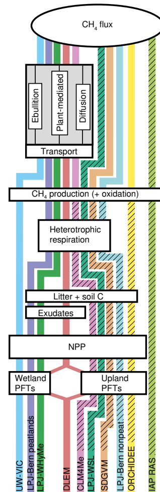
Fig. 7. Conceptual overview of the pathways from the carbon source to “ \text{CH}_4 flux” ( \text{CH}_4 flux per \text{m}^2 of wetland) in the participating models. Each model (and in some cases, version) is represented by a different colour. The flow of a particular model starts with the model’s name. The hatching of the lines indicates that the \text{CH}_4 model is not influenced by wetland hydrology (beyond changes in extent). “Wetland PFTs” means that the model uses wetland-specific PFTs, whereas “Upland PFTs” indicates that the model uses the already existing PFTs used for upland ecosystems. “NPP” stands for net primary production, “Exudates” are root exudates carbon pool. All models but the IAP-RAS model use NPP as a precursor of the carbon used directly in \text{CH}_4 production or indirectly in \text{CH}_4 production by estimating “Litter and Soil C”, “Exudates”, and “Heterotrophic respiration”. The models then calculate “ \text{CH}_4 production” and the oxidation based on the equations given in Table 5. Some models include the effect of “Transport” mechanisms explicitly, whereas others include transport only implicitly by either producing less \text{CH}_4 or oxidizing it before emitting it to the atmosphere. All models use some sort of temperature dependence when calculating NPP, heterotrophic respiration, and/or \text{CH}_4 production. In this figure, “LPJ-Bern nonpeat” includes both wetlands and wetsoils, which also incorporate plant exudates (graphical simplification).
