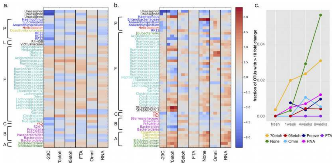
FIG 5 Distribution of the bacterial taxa that exhibit the greatest log fold changes in mean relative abundance. Heat maps show the \log_2 fold changes of the top 50 taxa that either increase (shown in red hues) or decrease (shown in blue hues) (a) once exposed to a preservation method (for 1 week at -20^\circ\text{C} and a few hours in the other preservatives) and (b) over time within a preservation method (from left to right: 1, 4, and 8 weeks, except for -20^\circ\text{C} , for which the 4- and 8-week time points are shown). Taxa are grouped by bacterial phyla (A, Actinobacteria ; B, Bacteroidetes ; C, Cyanobacteria ; F, Firmicutes ; L, Lentisphaeria ; P, Proteobacteria ) and colored by bacterial class. (c) A line graph shows the total fraction of OTUs that show a greater than 10-fold change in relative abundance for each stabilization method at each time point compared to the fresh sample. 70etoh and 95etoh, 70% and 95% ethanol, respectively.
