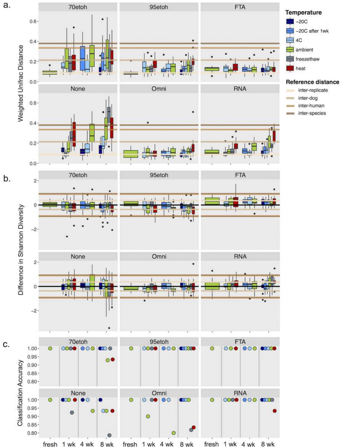
FIG 3 Summary of community changes by treatment over time. (a) Box plots show weighted UniFrac distances between treated samples and fresh samples taken on the day of sampling with no preservative. Horizontal lines show the average distance between replicate samples (lowest line, light tan), between different dogs (next line up, tan), between human individuals (next line up in dark tan), and between dogs and humans (highest line, brown). 70etoh and 95etoh, 70% and 95% ethanol, respectively. (b) Difference in alpha diversity is shown between samples indicated and the fresh sample. Reference absolute distances (interreplicate, interindividual, and interspecies) are shown in both the positive and negative directions. Note that the reference lines for interdog and interreplicate distances overlap significantly, as well as the lines for interhuman and interspecies distances. (c) The value shows the proportion of samples that were correctly assigned to the right individual using a random forest classifier. Colors represent the different temperatures at which samples were stored. “-20C following 1 week” represents samples that were stored at -20°C following 1 week of storage at ambient temperature.
