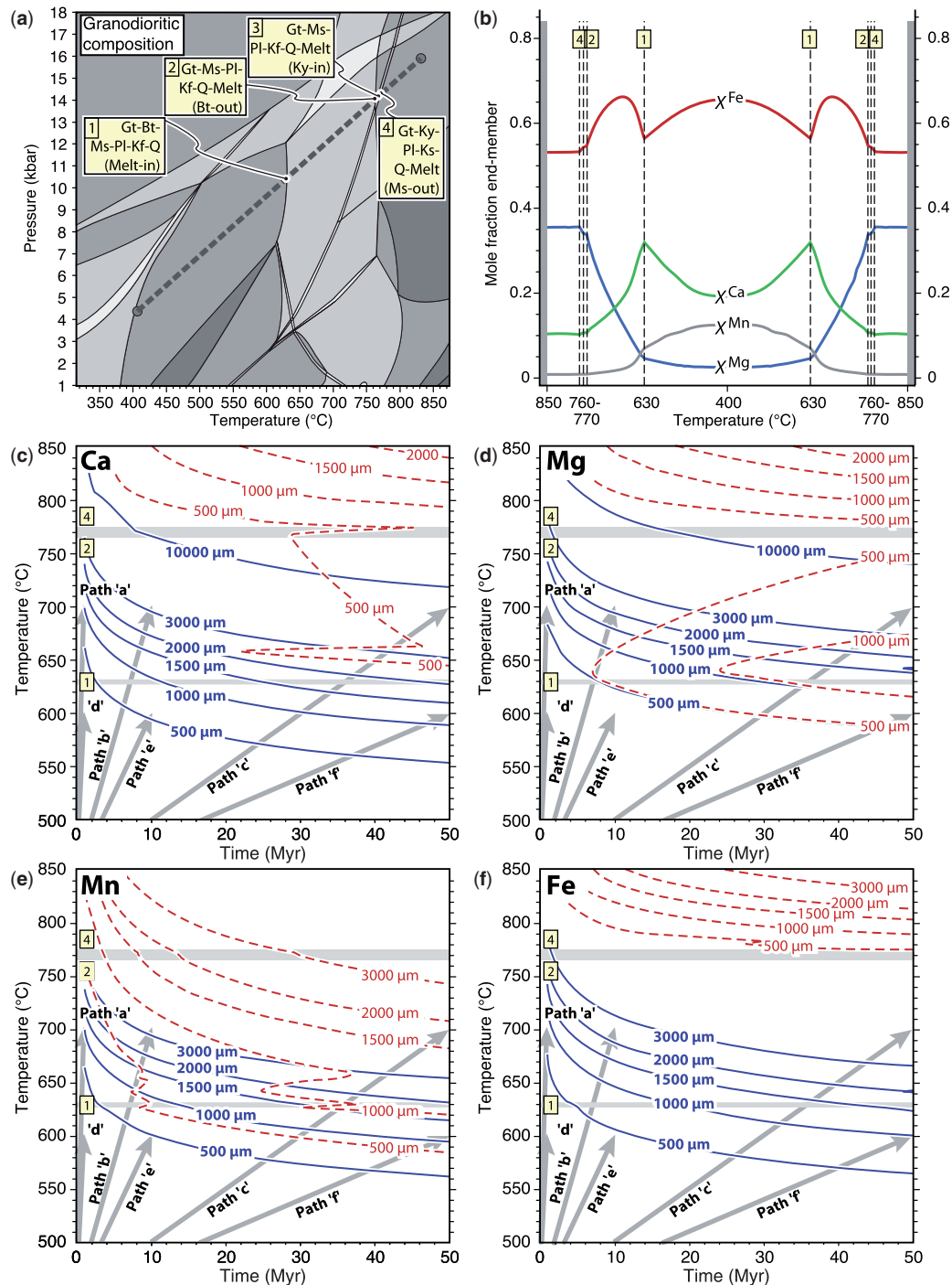
Fig. 6. Contoured results of modeled zoned garnet growth and diffusion during burial and heating of a granodioritic rock composition (Bohemian massif, sample KA-45b, Hradecký et al. , 2000) from 400 ^{\circ}\text{C} , 4.5 kbar. (a) P - T pseudosection showing equilibrium mineral assemblages in this bulk-rock composition. Assemblage boundaries along model P - T path (bold dashed line) are numbered 1-4 and labelled with the stable phases plus the change (phase-in or phase-out) upon heating. Other assemblage labels have been removed for clarity (available as Supplementary Data). It should be noted that the diagram is calculated for a fixed bulk-rock composition and would not be fully valid if mass was fractionated from the bulk into growing porphyroblasts along any specific P - T path. (b) Profile through the core of a spherical garnet crystal showing the chemical zoning developed during heating to 850 ^{\circ}\text{C} if diffusional relaxation does not occur. Zoning discontinuities form at assemblage boundaries [numbers 1-4 as in panel (a)]. Model crystals grow from a central core, so the x -axis (radial distance) equates to temperature of growth. (c) Plot of T_{\text{MAX}} reached during heating and the time required to achieve that temperature at a constant heating rate. Contours (continuous lines with bold labels in micrometres) show crystal diameters below which final core Ca (grossular) content is diffusionally modified from its initial growth value (see Appendix III, and discussion of calculation method in text). Dashed contours with labels in micrometres denote diameters of crystals that are effectively unzoned with respect to Ca (grossular) at the end of the simulation. Horizontal grey stripes represent discontinuities at mineral reactions (1)-(4) [as in (a) and (b)]. Grey arrows (labelled paths a-f) represent possible heating paths to 600 or 700 ^{\circ}\text{C} in 1, 10 or 50 Myr, as a result of rapid or slow orogenic events (as in Fig. 1). (d-f) T_{\text{MAX}} - t_{\text{TOTAL}} plot as (c) but showing contours for re-equilibration of Mg-pyrope (d), Mn-spessartine (e) and Fe-almandine (f) contents.
