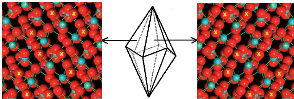
FIGURE 3. Adjacent crystal faces of calcite's common trigonal scalenohedral form have mirror-related surface structures (Hazen et al. 2001; Hazen 2004). Chiral surface structures of the (\bar{3}14) face (left) and the (214) face (right), which feature exposed O (X) and Ca (+) atoms, preferentially adsorb L- and D-aspartic acid, respectively.
