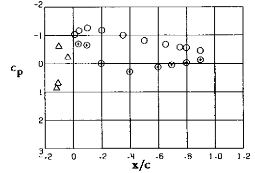
Station 7, y/(b/2) = 0.851
