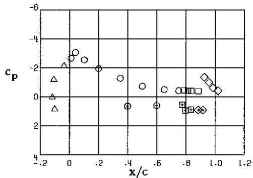
Station 5, \gamma/(b/2) = .652
