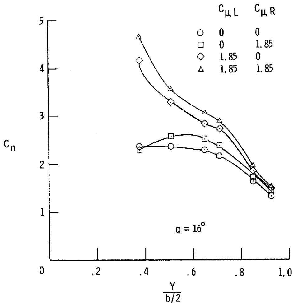
Figure 20. - Effect of an engine inoperative on span loading of the left wing.
