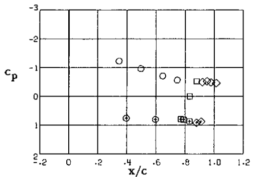
Station 2, \gamma/(b/2) = .301
