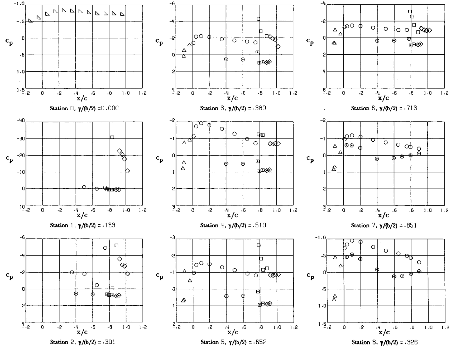
Figure 13. - PRESSURE DISTRIBUTIONS ON WING AND FLAP OF MODEL. C_{\mu L} = 1.85 , C_{\mu R} = 0
