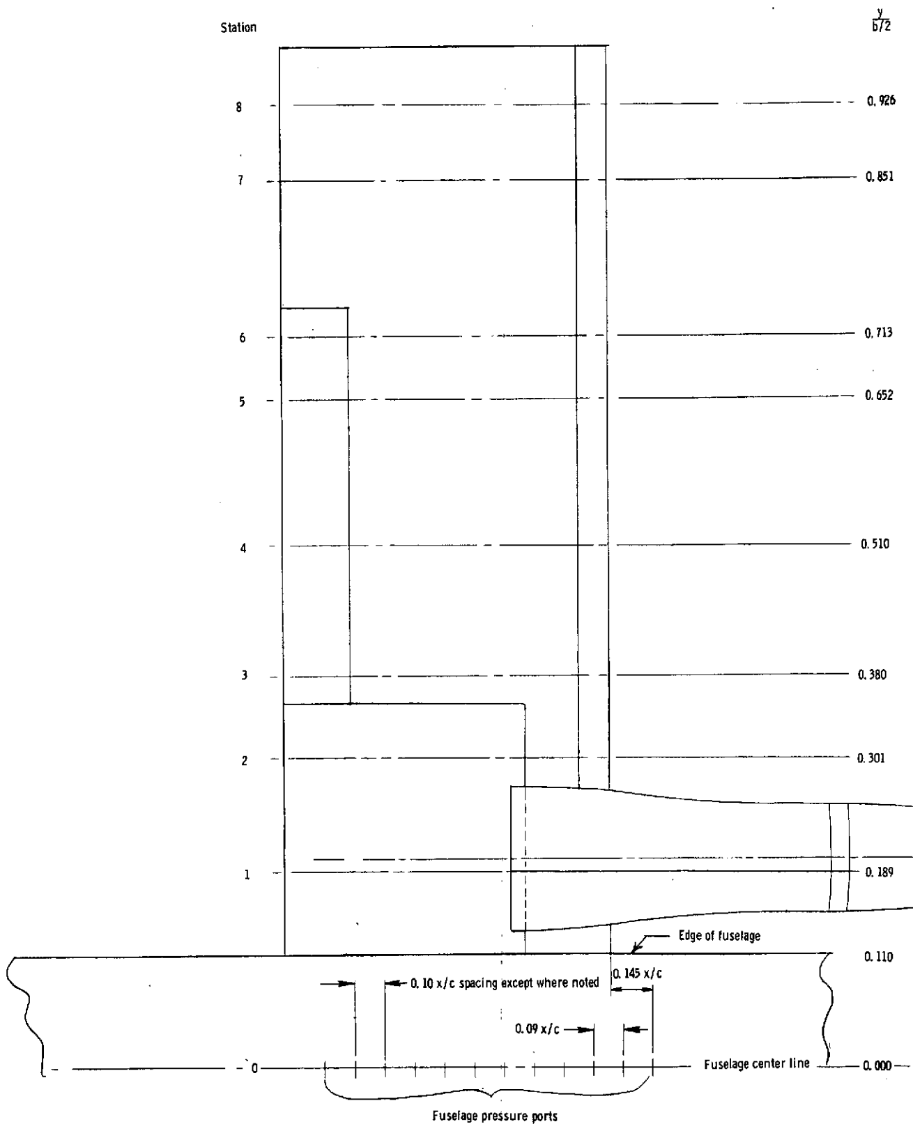
Figure 5. - Spanwise location of pressure orifices.
