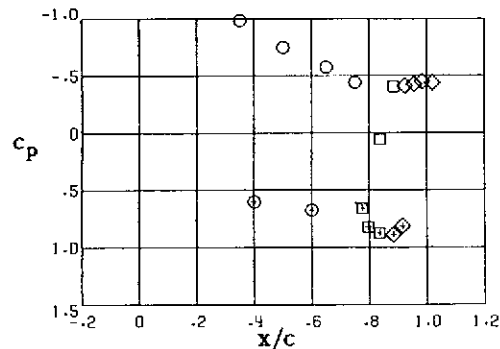
Station 2, y/(b/2) = -0.301
