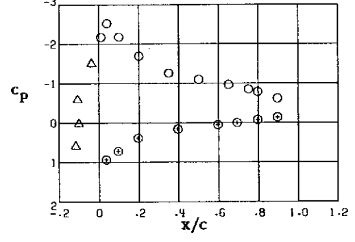
Station 8, y/(b/2) = -0.926
