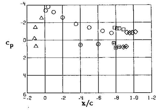
Station 6, \gamma/(b/2) = .713
