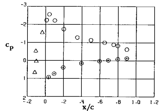
Station 8, \gamma/(b/2) = -0.926
