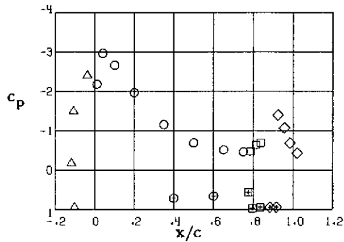
Station 4, \gamma/(b/2) = .510
