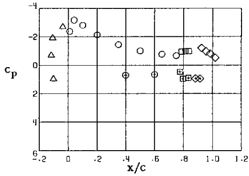
Station 4, y/(b/2) = -.510
