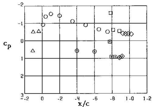
Station 3, y/(b/2) = -0.380
