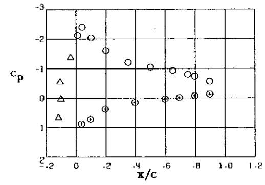
Station 8, \gamma/(b/2) = .926
