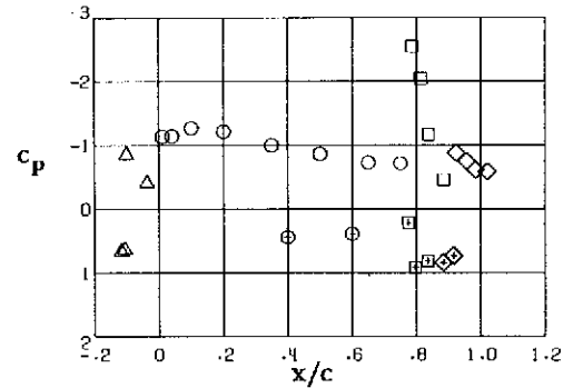
Station 6, y/(b/2) = -0.713
