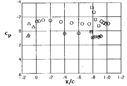
Station 6, y/(b/2) = 0.713
