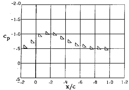
Station 0, \gamma/(b/2) = 0.000
