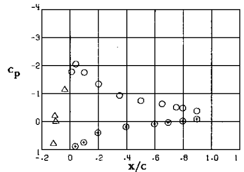
Station 8, \gamma/(b/2) = .926
