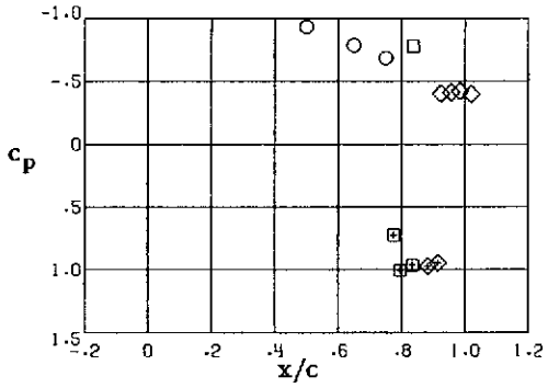
Station 1, y/(b/2) = -.189
