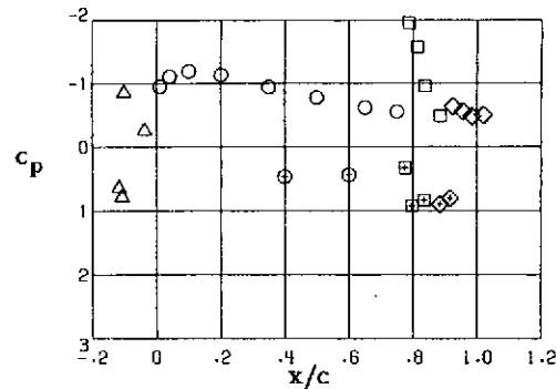
Station 6, y/(b/2) = -0.713
