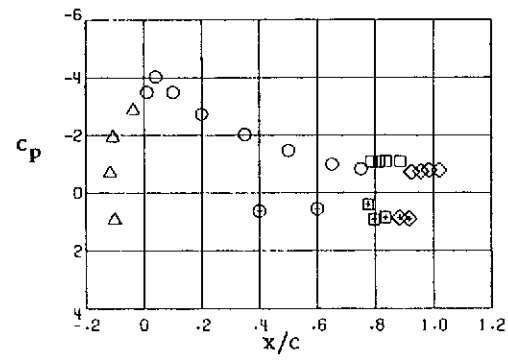
Station 5, \gamma/(b/2) = .652
