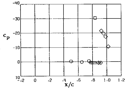
Station 1, y/(b/2) = 0.189
