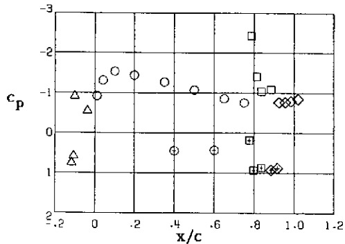
Station 5, y/(b/2) = 0.652
