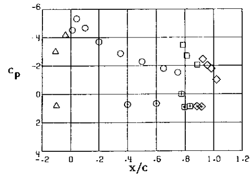
Station 3, \gamma/(b/2) = .380
