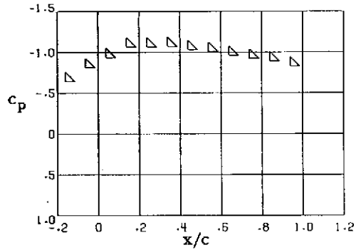
Station 0, y/(b/2) = 0.000
