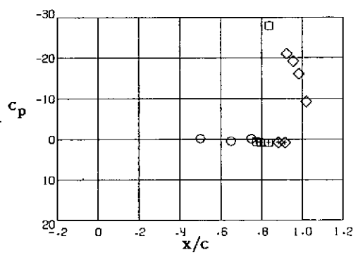
Station 1, \gamma/(b/2) = .189
