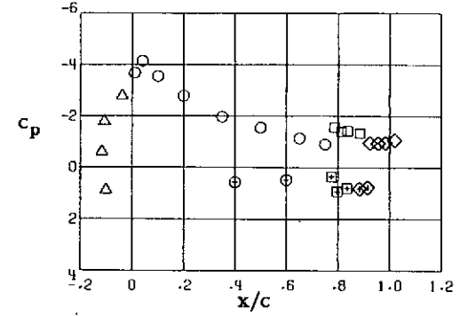
Station 6, \gamma/(b/2) = -0.713
