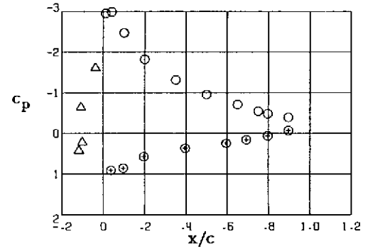
Station 7, y/(b/2) = -.851
