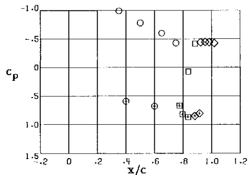
Station 2, y/(b/2) = -0.301
