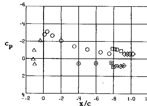
Station 6, y/(b/2) = 0.713
