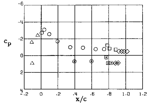
Station 3, \gamma/(b/2) = .380
