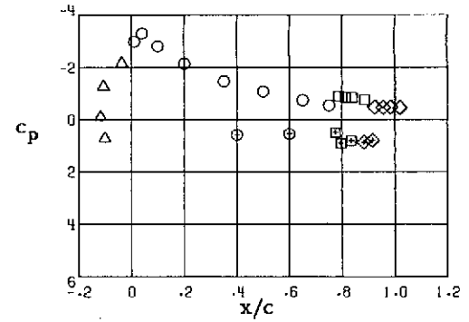
Station 6, y/(b/2) = -.713
