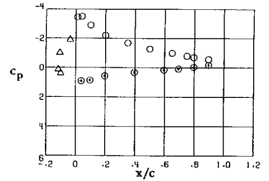
Station 7, \gamma/(b/2) = -0.851
