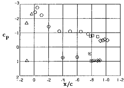
Station 3, y/(b/2) = -.380
