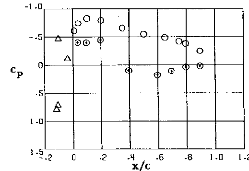
Station 8, y/(b/2) = -0.926
