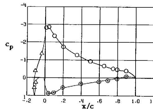
Station 7, y/(b/2) = 0.851
