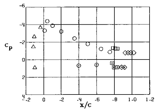
Station 4, \gamma/(b/2) = .510
