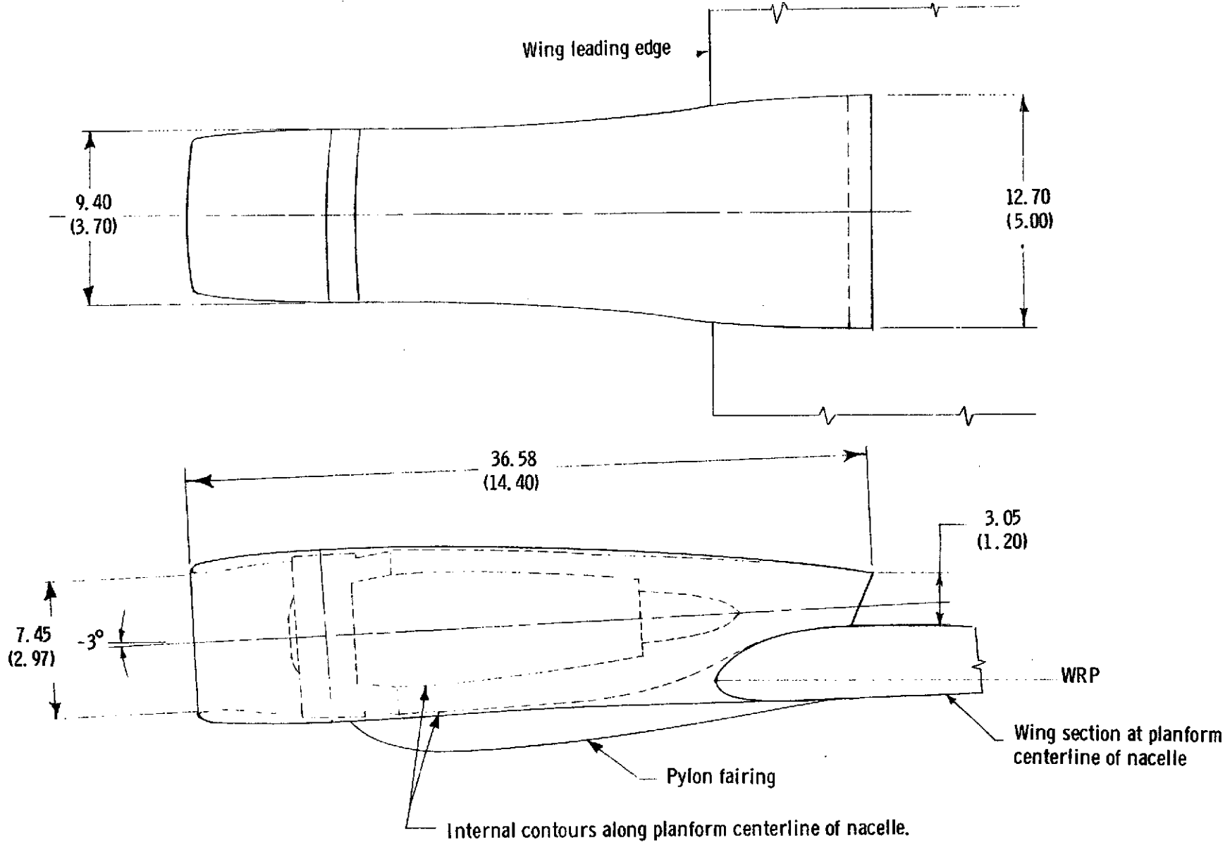
Figure 2. - Sketch of basic nacelle showing typical installation on wing.
