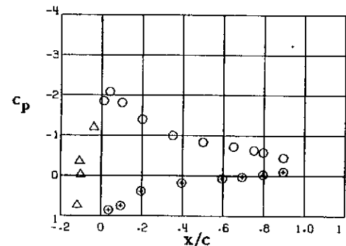
Station 8, y/(b/2) = 0.926
