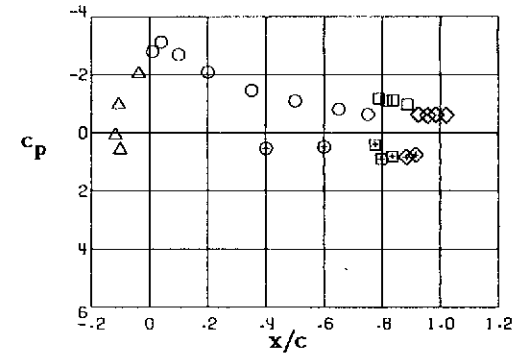
Station 6, y/(b/2) = -0.713
