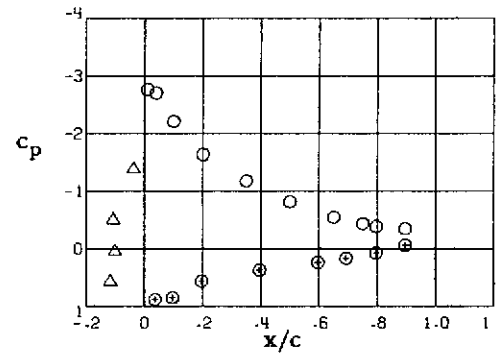
Station 7, \gamma/(b/2) = .851
