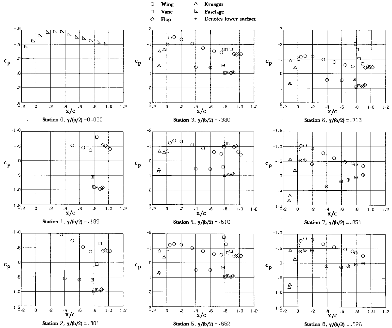
Figure 16. PRESSURE DISTRIBUTIONS ON WING AND FLAP OF MODEL WITH METAL FLAP BEHIND THE LEFT ENGINE REMOVED. C_{\mu L} = 0 , C_{\mu R} = 0 .
