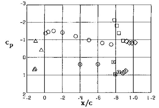
Station 6, y/(b/2) = -0.713
