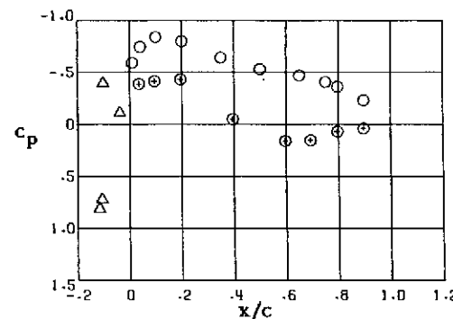
Station 8, y/(b/2) = -0.926
