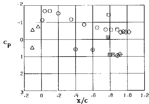
Station 3, y/(b/2) = -0.380
