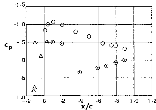
Station 7, y/(b/2) = -0.851
