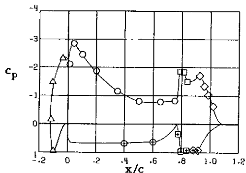
Station 4, y/(b/2) = 0.510
