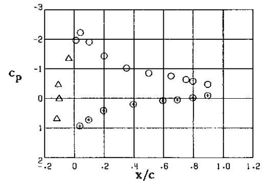
Station 8, y/(b/2) = -.926
