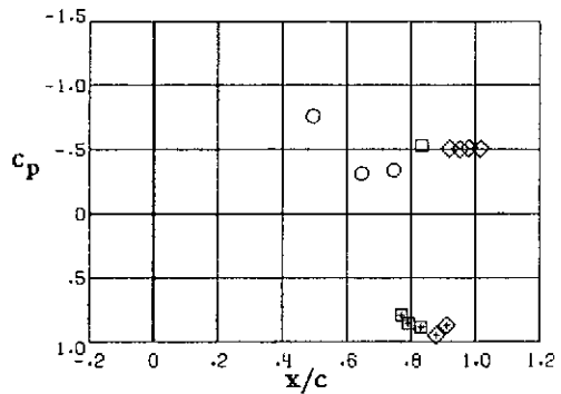
Station 1, \gamma/(b/2) = .189
