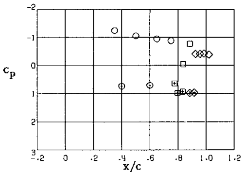
Station 2, y/(b/2) = -.301
