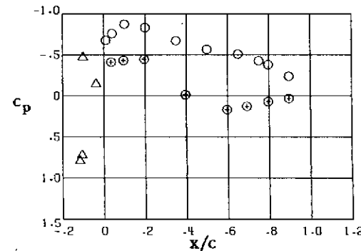
Station 8, y/(b/2) = -0.926
