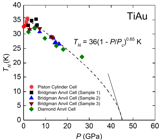
FIG. 7. (Color online) (a) A temperature vs pressure ( T_N vs P ) phase diagram for TiAu showing the extrapolated T_N(P) boundary (dashed curve) toward a critical pressure P_c at T = 0 K. The critical scaling function T_N = T_{N(P=0)} \times (1 - P/P_c)^\alpha was fit to the T_N(P) data up to P = 27 GPa. The ambient pressure value of the Néel temperature ( T_{N(P=0)} ) was set to 36 K while a rough estimate of the value for the critical pressure was determined from the fit to be P_c = 45 \pm 11 GPa. The value for the scaling exponent \alpha was determined from the fit to be \alpha = 0.65 \pm 0.20 . The slope of the curve near T_N = 0 K (represented by the solid black line) is dT_N/dP \sim -2.5 \text{ K GPa}^{-1} , while the slope of the nearly linear T_N(P) data accumulated from the various pressure cells up to P = 27 GPa is dT_N/dP = -0.59 \text{ K GPa}^{-1} .
