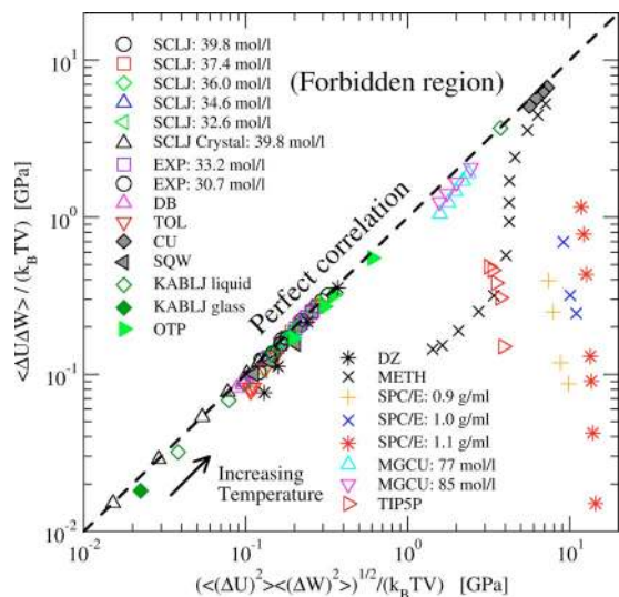
FIG. 10. (Color online) W, U -correlations for all simulated liquids; \langle \Delta W \Delta U \rangle / (k_B T V) plotted vs ((\langle \Delta W \rangle)^2 \langle (\Delta U)^2 \rangle)^{1/2} / (k_B T V) . Both quantities correspond to a pressure, which is given in units of GPa; for model systems not specifically corresponding to real systems, such as SCLJ, KABLJ, and SQW, argon units were used to set the energy and length scales. If the correlation is perfect ( R=1 ) the data fall on the diagonal marked by a dashed line. For the TIP5P model of water only temperatures with R > 0 are included; volumes were chosen to give a pressure close to zero.
