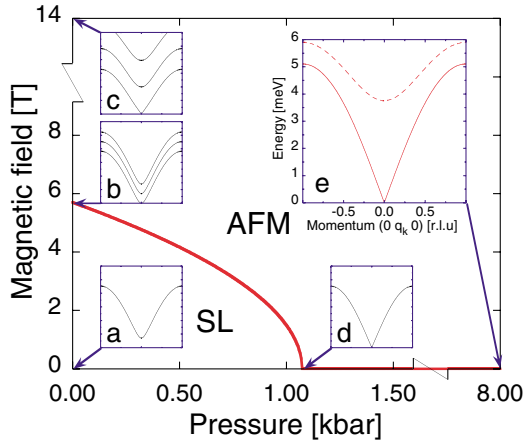
FIG. 1 (color). Magnetic field versus pressure phase diagram for the dimer compound \text{TiCuCl}_3 at T = 0 K. A square root phase boundary separates the spin-liquid (SL) phase from the AFM phase. Insets: Spin dynamics around the AFM zone center [7,8], \mathbf{Q} = \mathbf{q} + \boldsymbol{\tau} = (0 \ q_k \ 0) + (0 \ 4 \ 0) in reciprocal lattice units (r.l.u.). Common scale for (a)-(e), possible anisotropy gaps are not considered. (a) Degenerate triplet modes [12,13]. (b) Zeeman split triplet modes at H_c [21]. (c) Spin dynamics in the field-induced ordered phase [5]. (d) Degenerate and linear triplet modes close the spin energy gap at the critical pressure p_c . (e) Spin dynamics in the pressure-induced ordered phase. Two degenerate transverse Goldstone modes (solid line) and a longitudinal amplitude mode (dashed line) are expected [8].
