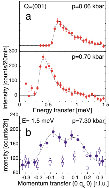
FIG. 3 (color). (a) Inelastic neutron scattering intensity in \text{TiCuCl}_3 at the AFM zone center \mathbf{Q} = \boldsymbol{\tau} = (0 \ 0 \ 1) r.l.u., p < p_c and T = 1.85 K. Elastic incoherent and inelastic background scattering measured away from the AFM zone center has been subtracted. (b) Constant-energy scan at E = 1.5 meV (solid circles), \mathbf{Q} = \mathbf{q} + \boldsymbol{\tau} = (0 \ q_k \ 0) + (0 \ 4 \ 0) r.l.u. and T = 1.5 K. To be compared with the corresponding scan at T = 30 K > T_N (open circles) and at the AFM zone boundary \boldsymbol{\tau} = (0 \ 3 \ 0) r.l.u. (open squares). Solid lines in (a) and (b) represent least-square fits including convolution with the full 4D resolution ellipsoid.
