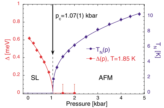
FIG. 2 (color). Pressure-induced quantum phase transition in \text{TiCuCl}_3 between SL and AFM phases. Singlet-triplet gap \Delta(p) and Néel temperature T_N(p) measured at \mathbf{Q} = \boldsymbol{\tau} = (0 \ 0 \ 1) r.l.u.
