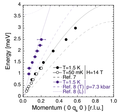
FIG. 4 (color). Spin dynamics in \text{TiCuCl}_3 measured at p = 7.3 kbar > p_c and H = 0 T compared with p = 0 kbar and H = 14 T > H_c [5], \mathbf{Q} = \mathbf{q} + \boldsymbol{\tau} = (0 \ q_k \ 0) + (0 \ 4 \ 0) r.l.u. The solid lines represent fits described in the text. Predictions from theory [7,8] are shown for the field-induced (dashed black line) and the pressure-induced ordered phase with transverse (T, dashed blue line) and longitudinal (L, dotted blue line) modes.
