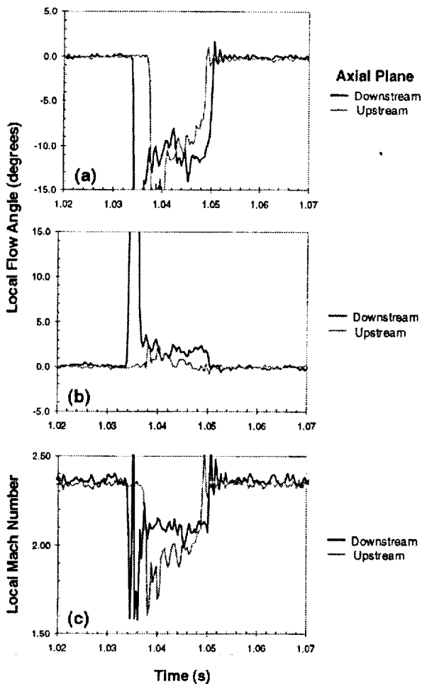
(a) Local pitch angle, \alpha (b) Local yaw angle, \beta (c) Mach number.
