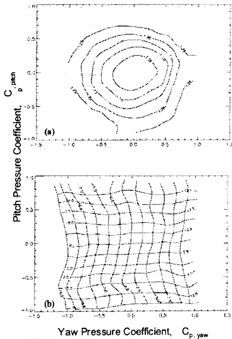
(a) Pitot pressure correction. (b) Flow angle calibration.
