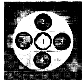
Figure 8. Front view of five-hole conical probe.
