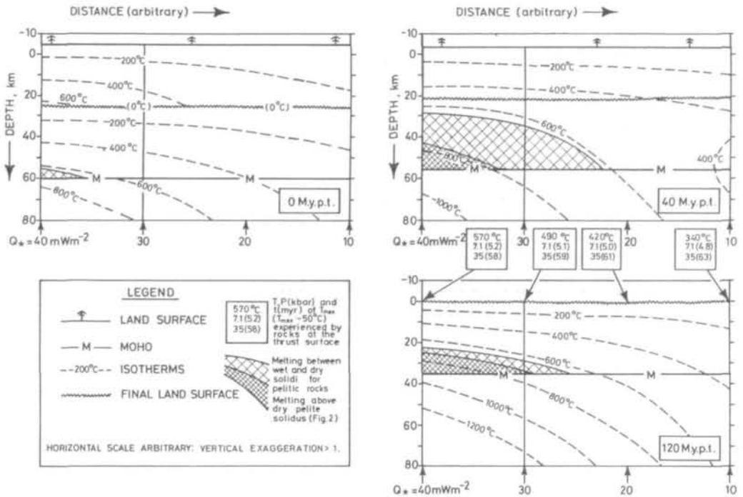
FIG. 9. As Fig. 8, except that the initial thrust thickness is a constant 30 km and it overrides a crust of 35 km; the thermal regime is as in Fig. 8, but the mantle heat flow varies from 40 \text{ mW m}^{-2} on the left to 10 \text{ mW m}^{-2} on the right.
