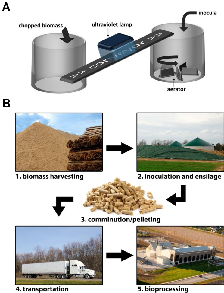
Figure 1. A possible scheme for incorporating biological pretreatment into biofuels manufacturing. A. Treatment to suppress the growth of endogenous microorganisms to allow establishment of the inoculated fungal culture. A variety of treatments could be utilized, including ultraviolet, microwave, or radio frequency treatment. This scheme is based on the successful biopulping inoculation strategy described by Scott et al. [66]. B. Overall scheme for biofuels production including biological pretreatment. (B.5. photo courtesy of Jay Grabiec, Eastern Illinois University).
