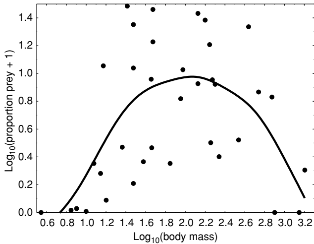
Fig. 2. Distance weighted least-squares relationship between mean percentage of lion Panthera leo diet ( \log_{10} + 1 ) and prey body mass ( 0.75 \times adult female body mass) ( r = 0.19 , P = 0.28 ).
