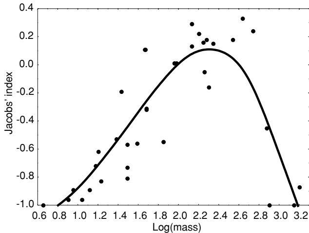
Fig. 3. Distance weighted least squares relationship between lion Panthera leo prey preference (mean Jacobs' index) and the \log_{10} of prey body mass ( r = 0.401 , P = 0.015 ).
