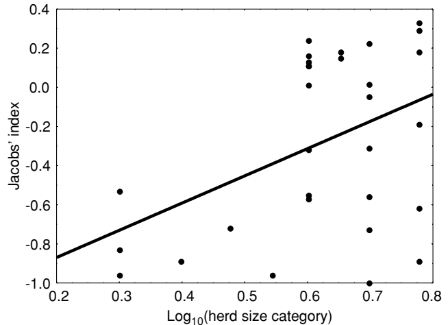
Fig. 5. Linear relationship between lion Panthera leo prey preference (mean Jacobs' index) and prey herd size ( r^2 = 0.186 , P < 0.017 , y = -1.15 + 1.39x ).
