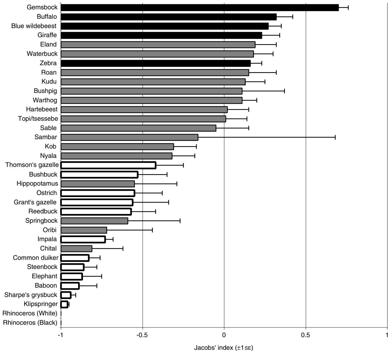
Fig. 1. Lion Panthera leo dietary preferences based on Jacobs' index (mean \pm 1 SE) of 48 lion populations at differing prey densities. Black bars, species taken significantly more frequently than expected based on their availability (preferred); grey bars, species taken in accordance with their relative abundance; unfilled bars, species taken significantly less frequently than expected based on their availability (avoided). Only species recorded in lion diet more than once are included.
