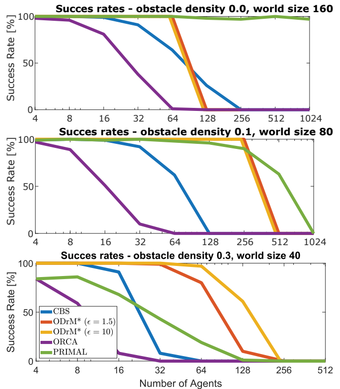
Figure 6. Success rates of the different planners in our three scenarios. PRIMAL outperforms all planners in the top obstacle-free world, slightly outperforms the others in low-obstacle-density worlds, and is strongly outperformed in the high-obstacle-density world.
