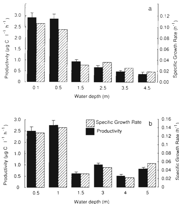
Fig. 5. Productivity and specific growth rates of bacteria in the water column on a rising tide at mid-tide height in transects from nearshore to 1 km offshore in autumn; water temperature 29 °C. Water depths at low tide are indicated. Duplicate determinations were made of both numbers and productivity; the range of variation is indicated for productivity. (a) Bay. Seagrass shoot density decreased with increasing water depth to 2.5 m. No seagrass was present below 3.5 m. (b) Reef flat. The reef crest was at 2 m depth. No seagrasses or macroalgae were present inside the reef crest at 1.5 m
