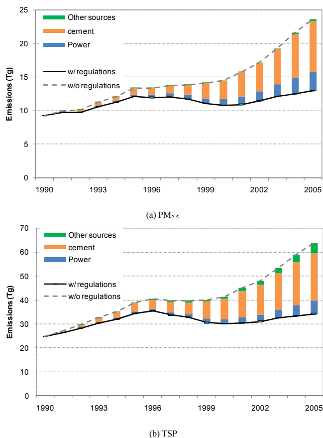
Fig. 15. Reductions of (a) PM_{2.5} and (b) TSP emissions due to improved emission control regulations and technologies from power sector, cement industry and other sources. The dark solid line denotes our estimates of inter-annual PM_{2.5} emissions in China, and the gray dashed line denotes the hypothetical PM_{2.5} emissions if penetration of PM control technologies remains at the 1990 level.
