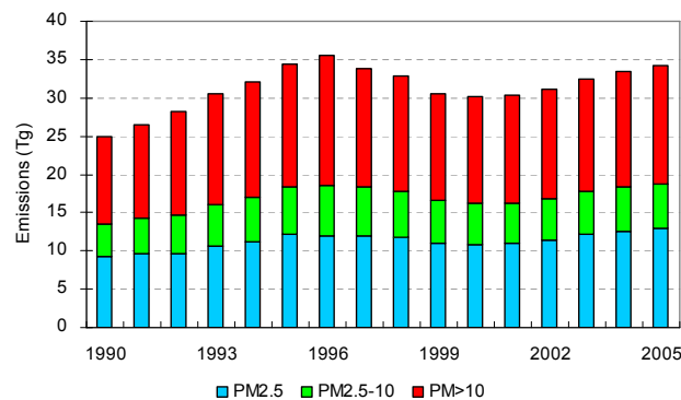
(a) total PM emissions
