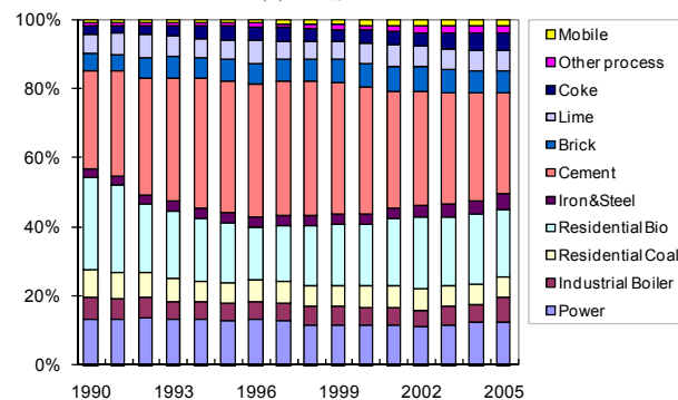
(c) \text{PM}_{10} emissions
