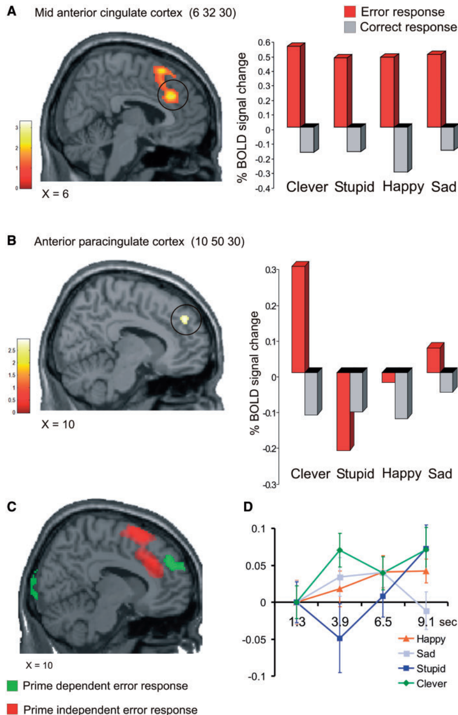
Fig. 3 (A) The activation in the mid anterior cingulate cortex represents error detection on the n -back task. There was no significant difference in this area between the four conditions [ P < 0.05 corrected conjunction analysis (Clever and Stupid and Happy and Sad)]. (B) The imaging data revealed a significant positive interaction in the anterior paracingulate cortex [ P < 0.02 corrected [(Clever + Sad) vs (Stupid + Happy)]]. Note that the BOLD pattern resembles the pattern of post-error RT for the different conditions. (C) Prime sensitive activation in the anterior paracingulate cortex (shown in green) lay anterior to that of medial prefrontal activation generally seen for error detection (shown in red). The SPMs are thresholded at P < 0.05 uncorrected. (D) The time course of activation is plotted for the four conditions at the event of making errors on the n -back task. The time series of the BOLD signals is taken at the coordinate 10 50 30. The plot represents the average value for the whole group, as well as the standard error of the mean.
