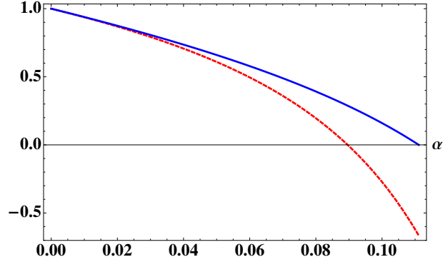
FIG. 2: A_{\dot{Q}_3^3} in Eq. (4.11) (dashed red) and A_{\dot{Q}_\sigma(\partial Q_\sigma)^2} in Eq. (4.12) (plain blue) as we vary \alpha with c_{\mathcal{D}}^2 \ll 1 .
