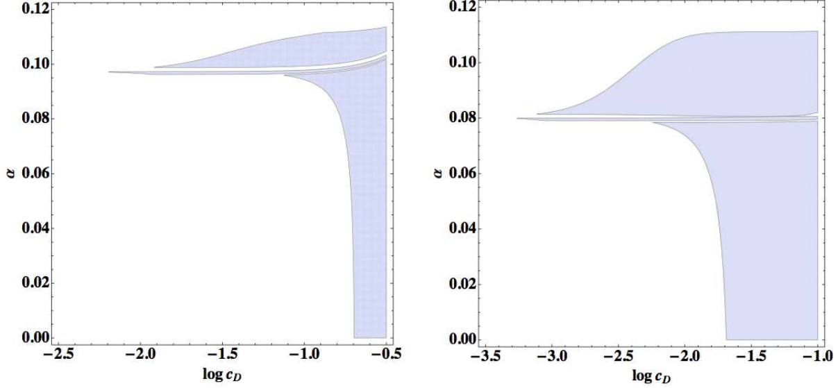
FIG. 6: The region in the parameter space (c_{\mathcal{D}}, \alpha) allowed by the observational constraints on f_{\text{NL}}^{eq} and f_{\text{NL}}^{orth} for T_{\sigma s} = 0 (left) and T_{\sigma s} = 10 (right).
