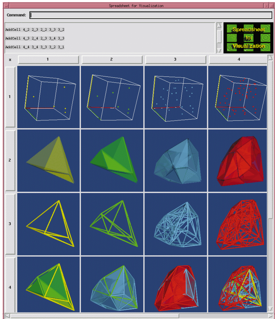
1 Visualization of 3D random-point generation and Delaunay triangulation of the resulting point set. The columns visualize the algorithm's outcome after 5, 6, 25, and 50 steps, respectively. The last row shows the result of several addition operations (the formula syntax is "command result operands"): AddCell 4_1 3_2 3_1 2_2 2_1; AddCell 4_2 3_3 3_2 2_3 2_2; AddCell 4_3 3_4 3_3 2_4 2_3; AddCell 4_4 3_4 3_3 3_2 3_1;
