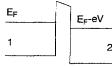
Figure 16 Planar potential barrier separating two degenerate electron gas regions of equal chemical potential, but with shifted Fermi levels because of the voltage V applied across the barrier
