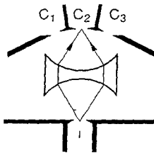
14. Experimental device used to demonstrate focusing of a ballistic electron beam (for an angle of incidence) and total reflection (for an angle of incidence greater than the critical angle) at a potential barrier defined electrostatically. A concave lens is positive, even though it is refracted away from the surface of a region with reduced phase velocity. In a convex lens, a ray is refracted towards the surface.
