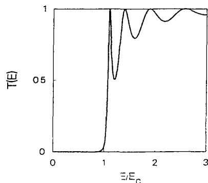
Figure 18 Transmission probability versus energy for a rectangular barrier of height E_c and thickness L , for the case that \hbar^2/2mL^2 = 0.01E_c . The curve has been calculated from Eqs (72) and (75)
