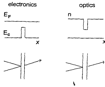
FIG. 15. a. Tunneling of an electron incident on a region of increased electrostatic potential (reduced momentum) at an angle such that classically it would be totally reflected. b. Frustrated total reflection of light incident on a region of reduced refractive index.
