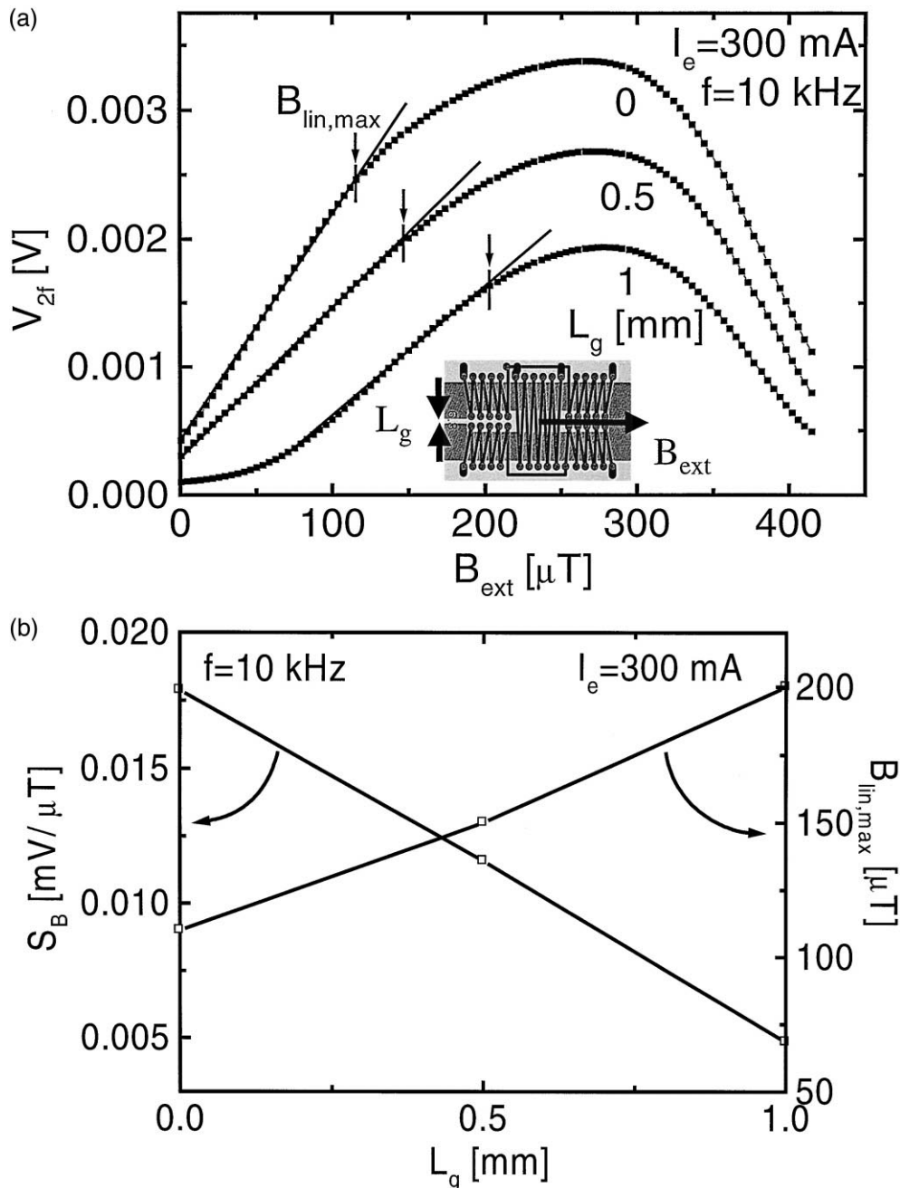
Fig. 3. (a) Second harmonic voltage V_{2f} of the detection coil of a rectangular fluxgate sensor as a function of B_{\text{ext}} for various gap length L_g at a frequency f = 10 kHz and for an excitation current I_e of 300 mA. (b) Sensitivity S_B = (dV_{2f})/(dB_{\text{ext}}) and maximum of the linear range B_{\text{lin,max}} , determined from the curves of a).
