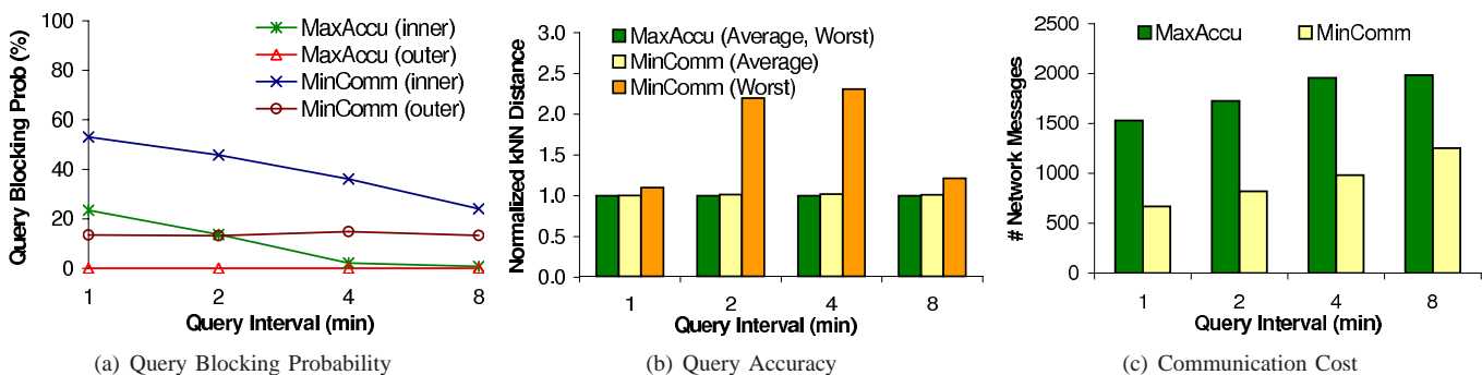
Fig. 15. Performance Comparison of Cloaking Algorithms
