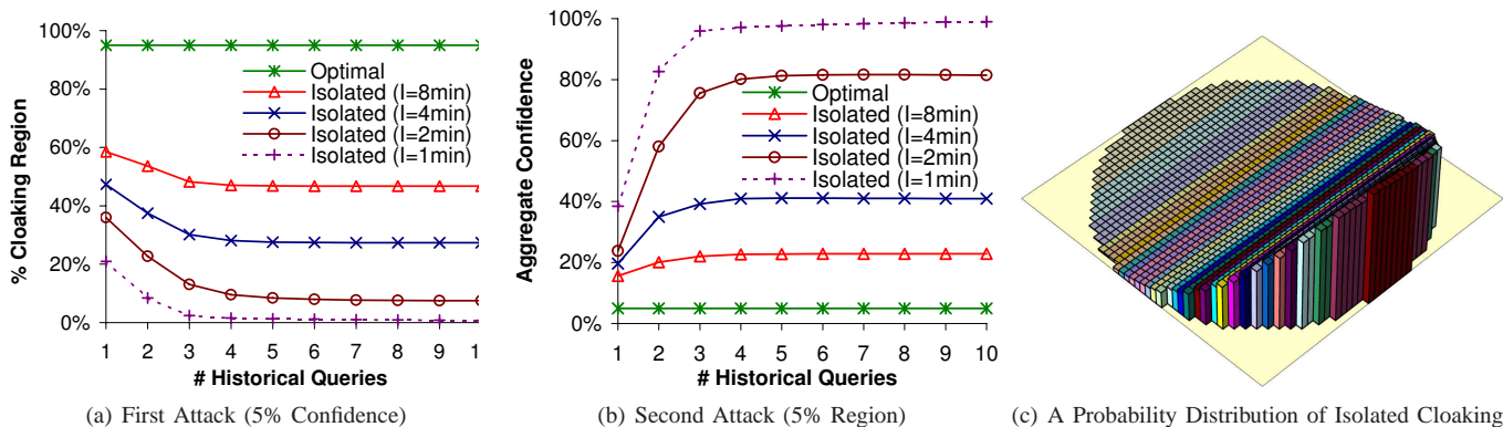
Fig. 14. Trace Analysis Attacks
