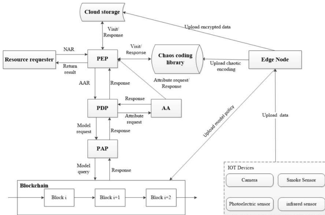
Fig. 6 Blockchain-based access control model
