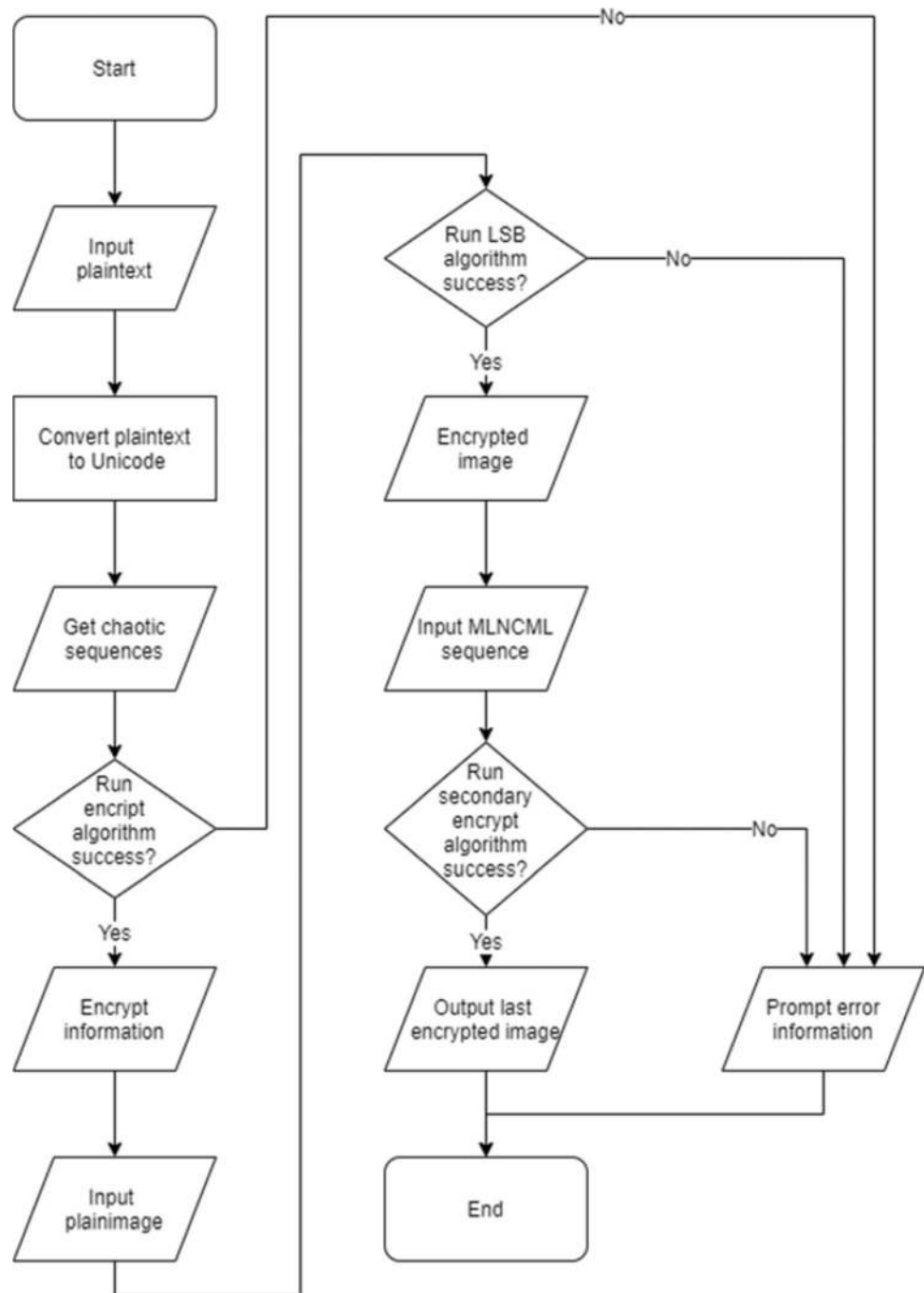
Fig. 5 LSB image encryption algorithm flowchart combined with MLNCML
